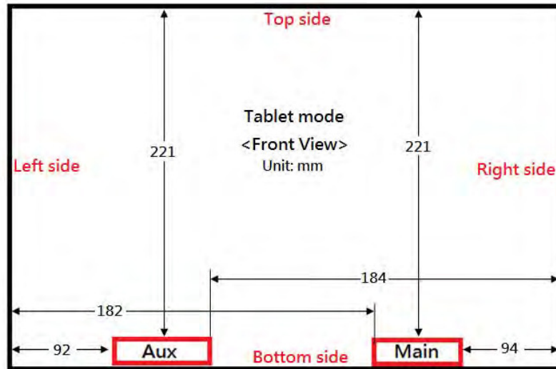
Fig.8 Antenna location of EUT (Tablet mode)
