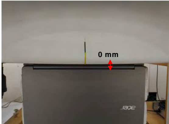
Fig.3 EUT Back side to flat phantom (Laptop mode)
