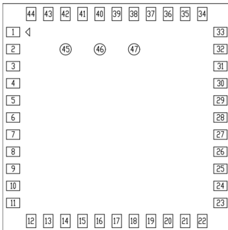
AW-CM467-USB Top View Pin Map
