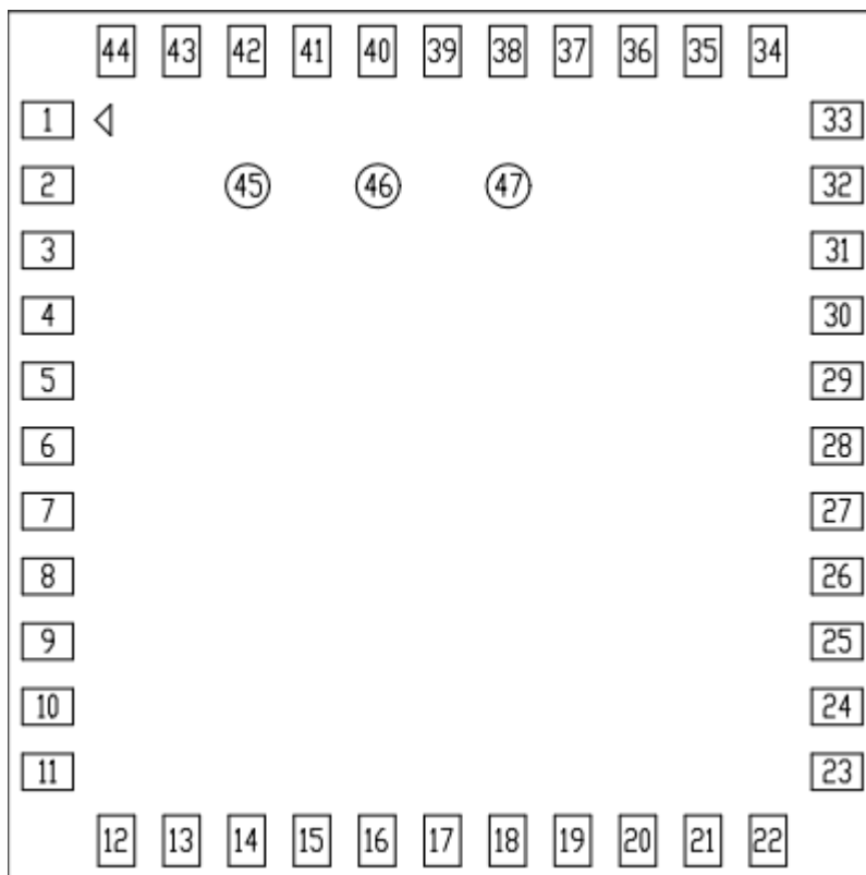
AW-CM467-USB-I Top View Pin Map
