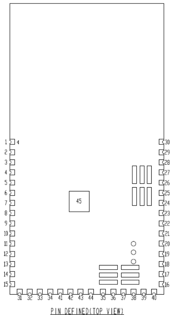
AW-CU639-ZC1 Pin Map (Top View)
