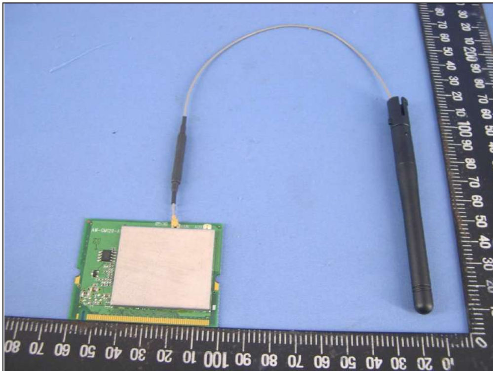
EUT with Antenna 2
