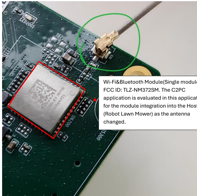
Wi-Fi&Bluetooth Module(Single module), FCC ID: TLZ-NM372SM
