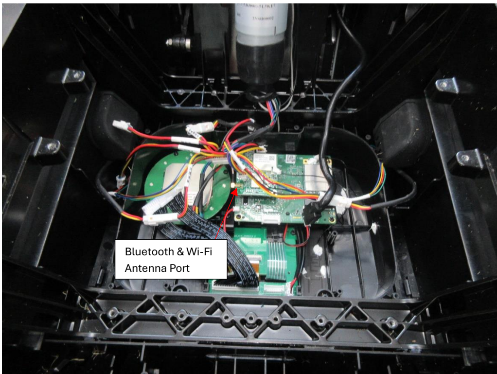
Internal View (Host: Lymow One)
