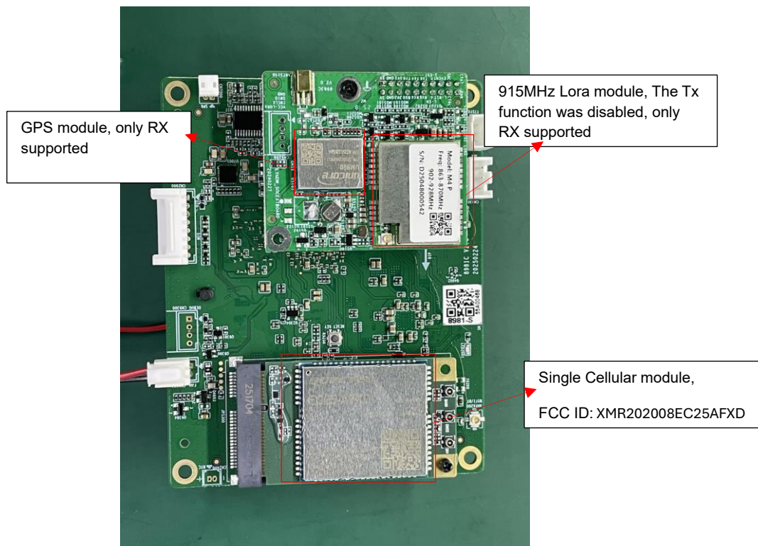
Internal View (Host: Lymow One)
