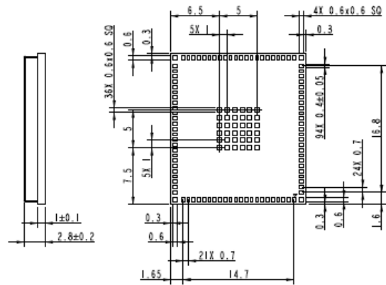
TOLERANCE UNLESS OTHERWISE SPECIFIED: \pm 0.1\text{mm}
