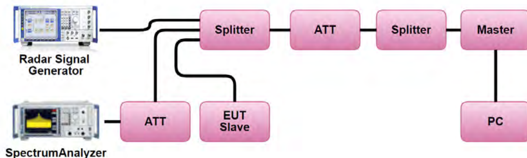
Client without Radar Detect Conducted Measurement
