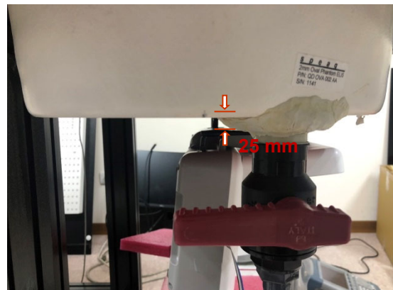
Photograph 8. Body, Back Edge of Antenna, 25mm
