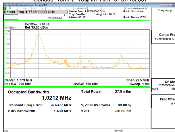
Band66_15MHz_16QAM_RB1_0_CH132597
