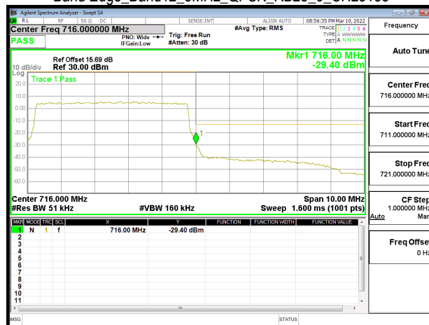
Band Edge_Band12_5MHz_QPSK_RB25_0_CH23155
