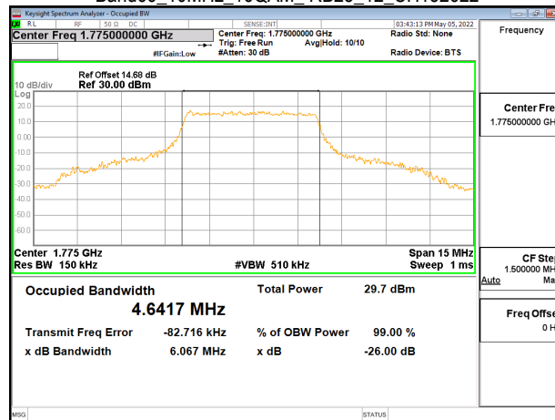
Band66_10MHz_16QAM_RB25_12_CH132622
