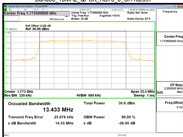
Band66_15MHz_QPSK_RB75_0_CH132597
