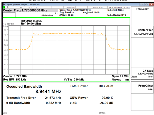
Band66_10MHz_QPSK_RB50_0_CH132622
