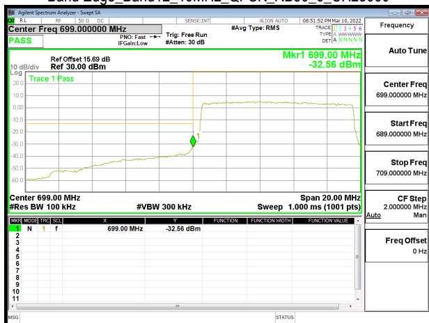
Band Edge_Band12_10MHz_QPSK_RB50_0_CH23060
