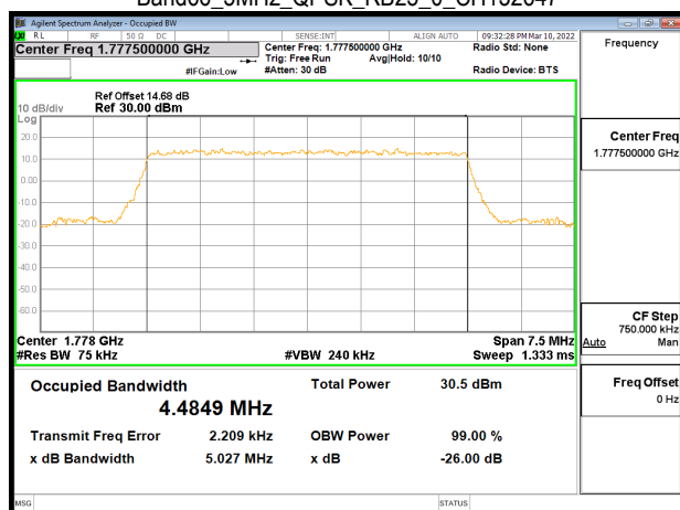
Band66_5MHz_QPSK_RB25_0_CH132647
