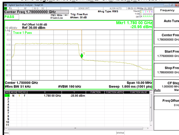
Band Edge_Band66_10MHz_QPSK_RB1_0_CH132022
