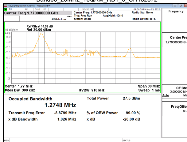
Band66_20MHz_16QAM_RB1_0_CH132572
