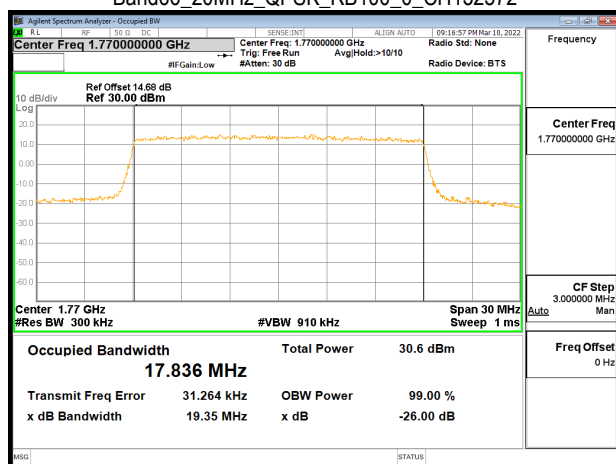
Band66_20MHz_QPSK_RB100_0_CH132572
