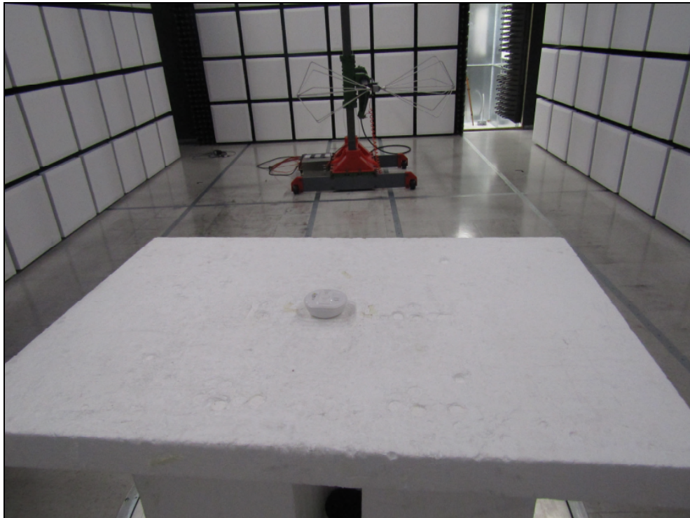
Figure 3: Radiated Emissions Below 1GHz – Rear View
