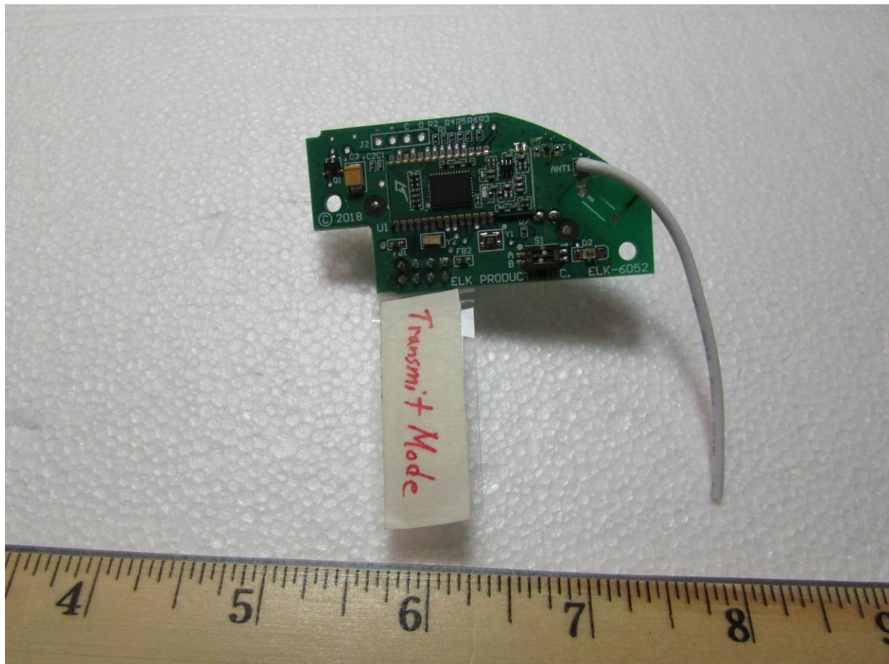
Figure 5: PCB Top
