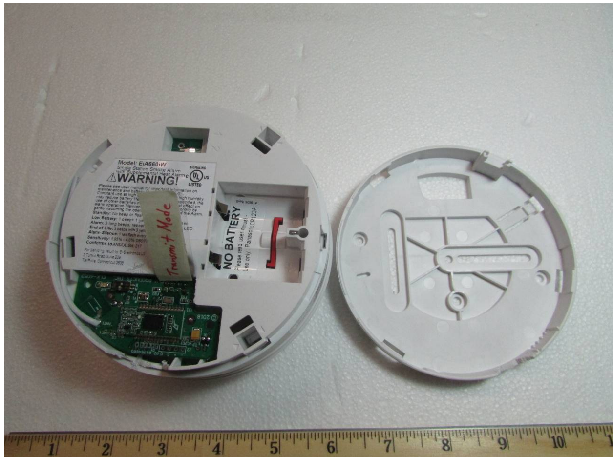
Figure 1: PCB in housing
