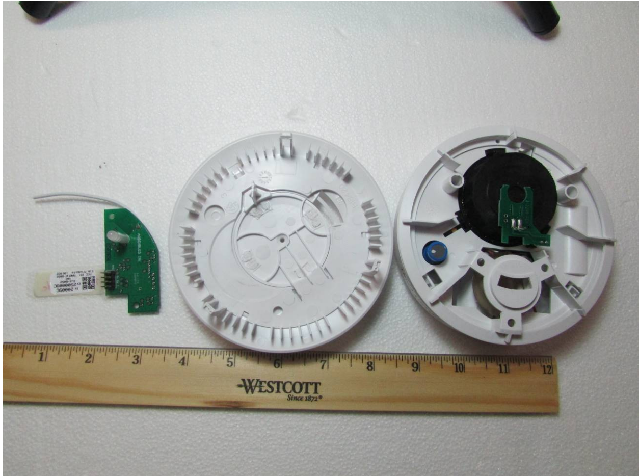
Figure 3: Top cover removed
