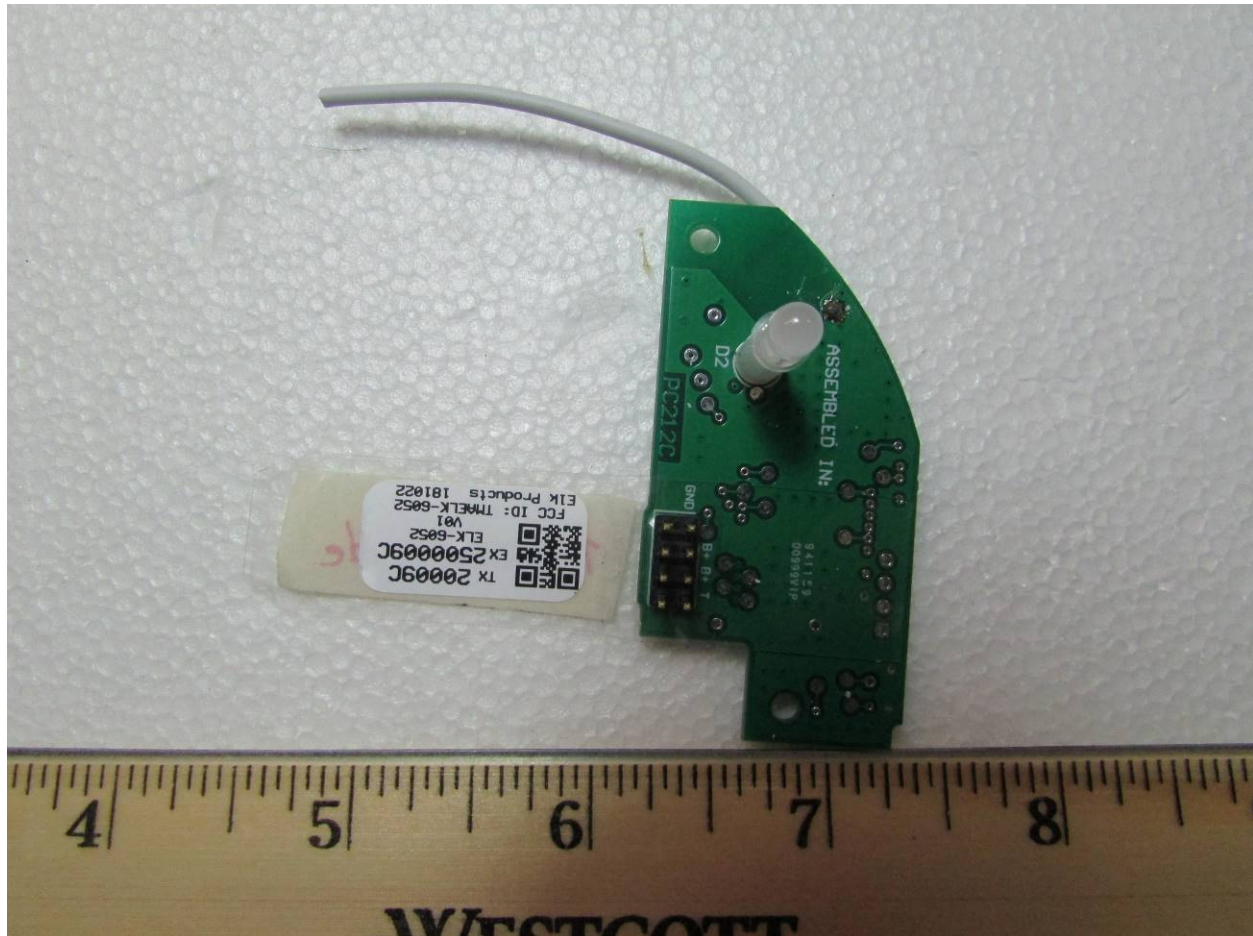
Figure 4: PCB bottom
