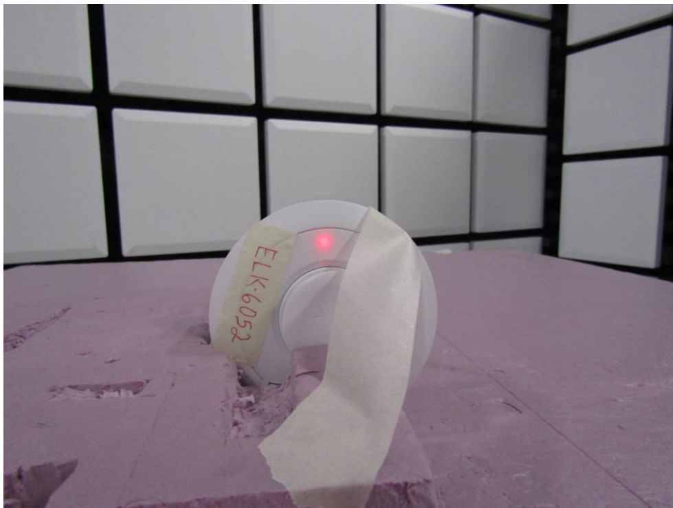
Figure 7: Radiated Emissions – Front – Above 1GHz - ZPOS
