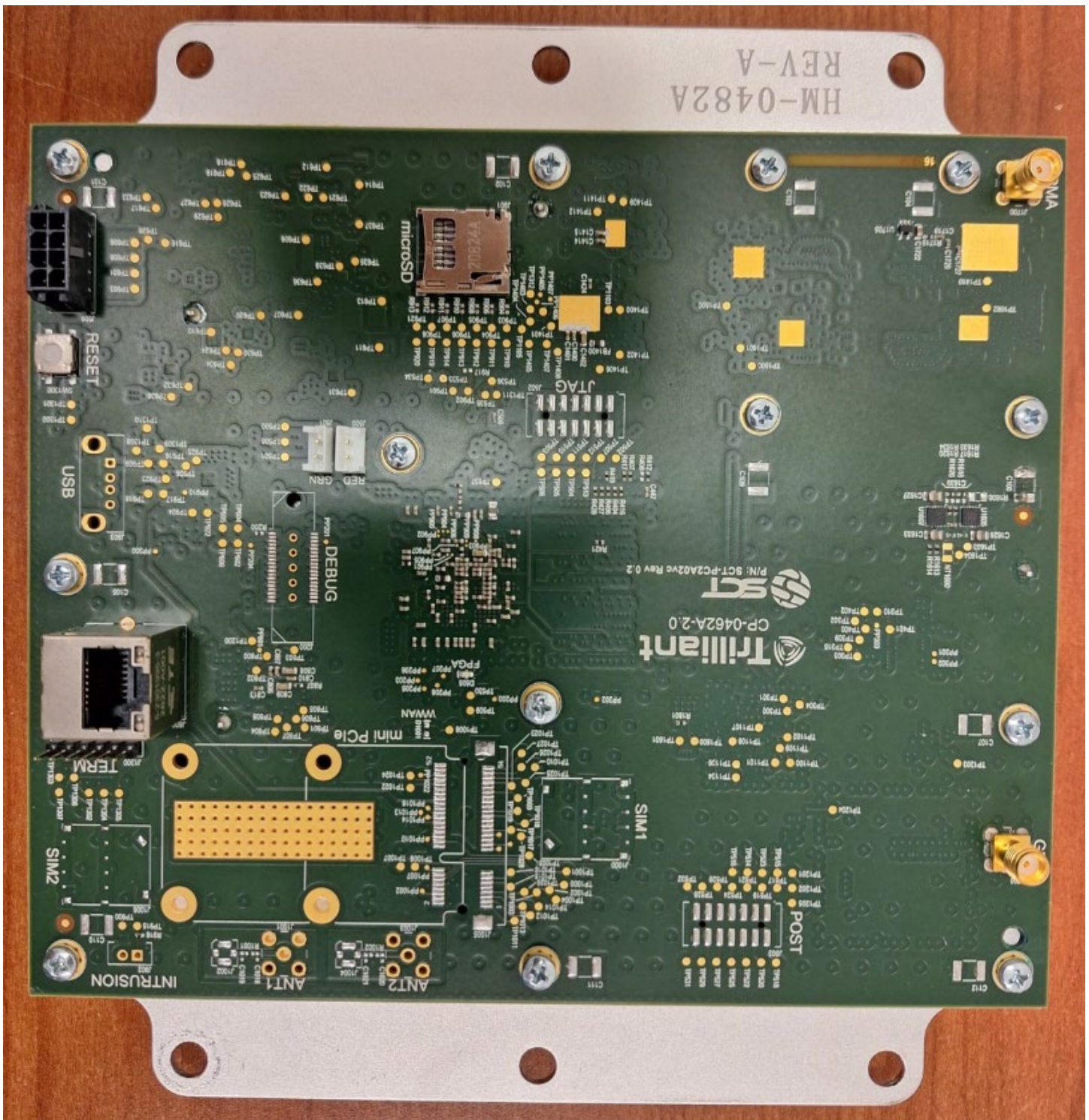
Pliny board and shield, top view
