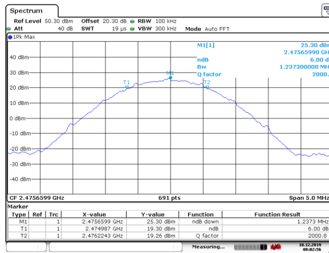
Figure 8.5-3: 6 dB bandwidth on high channel
