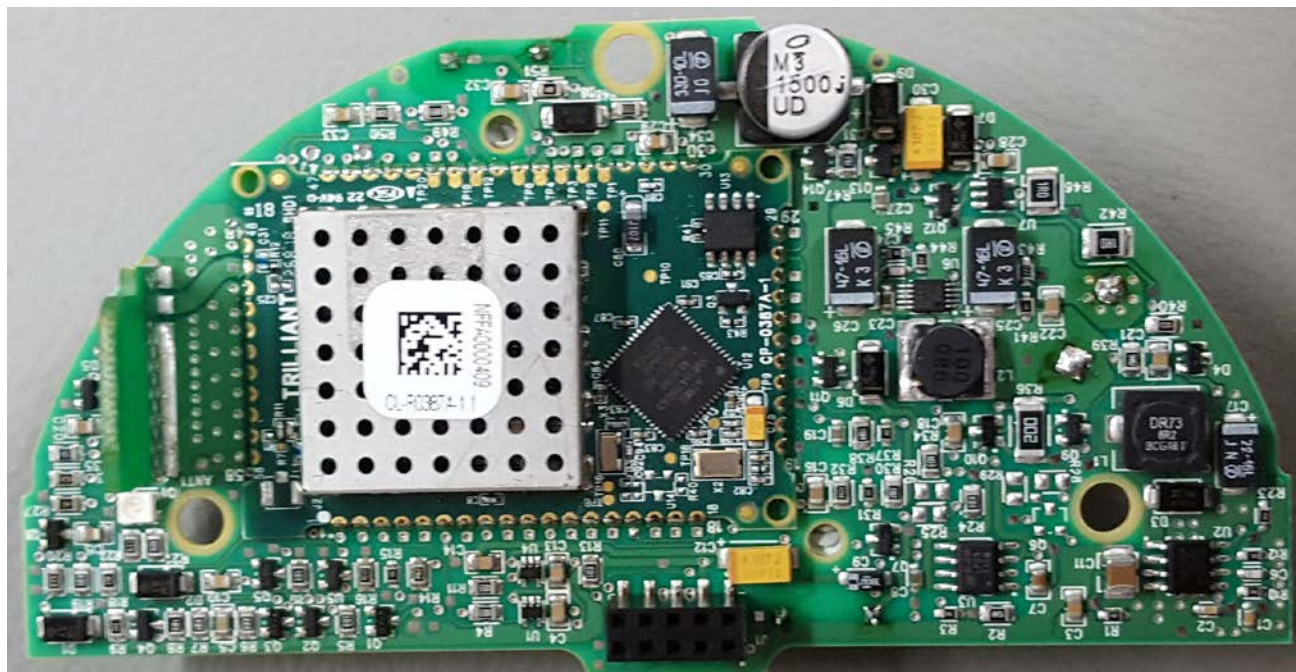
Top and bottom sides without shield of CP-0387A-1
