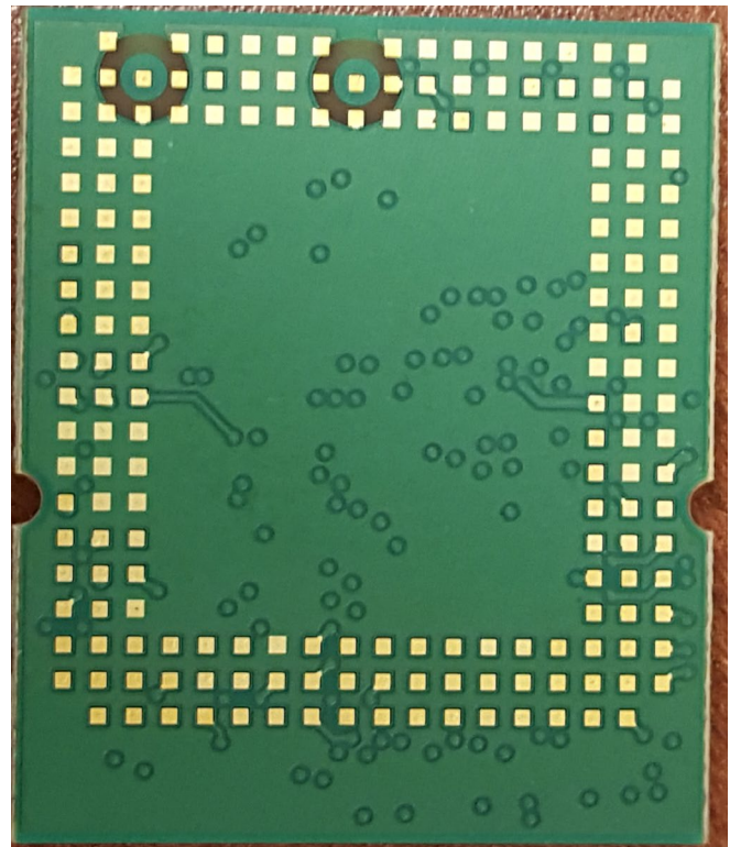
Top view (CL-R0368A-1.4 & CL-R0368B-1.2)
