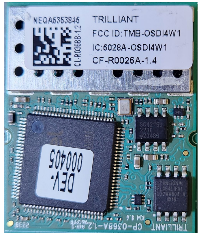
Top view (CL-R0368A-1.4 & CL-R0368B-1.2)
