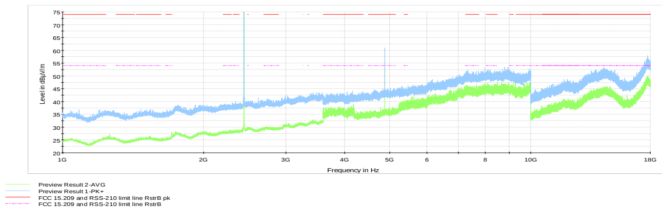
Figure 8.6-26: Cabinet radiated Spurious emissions 1to18 GHz, Tx @ mid channel
