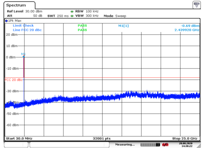
Figure 8.6-4: Conducted spurious emissions, tx on mid channel
