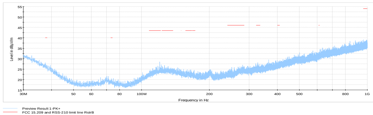
Figure 8.6-23: Cabinet radiated Spurious emissions within 30 to 1000 MHz, Tx @ mid channel
