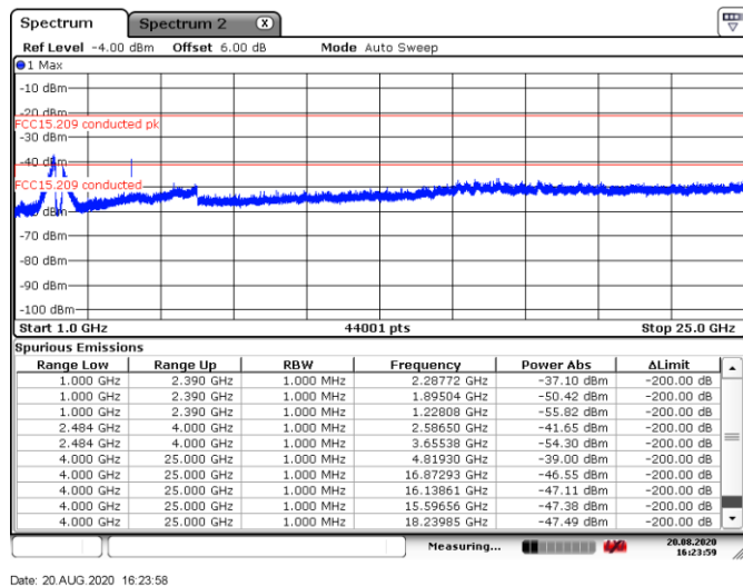
Figure 8.6-13: Conducted spurious emissions above 1 GHz within restricted bands, tx on low channel
