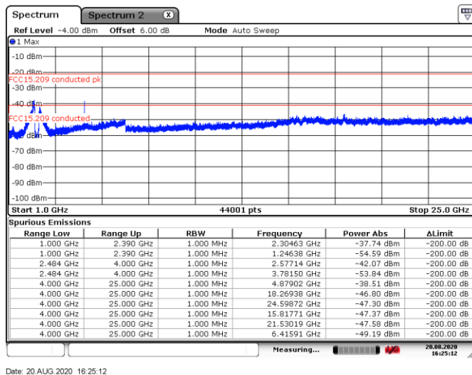
Figure 8.6-14: Conducted spurious emissions above 1 GHz within restricted bands, tx on mid channel
