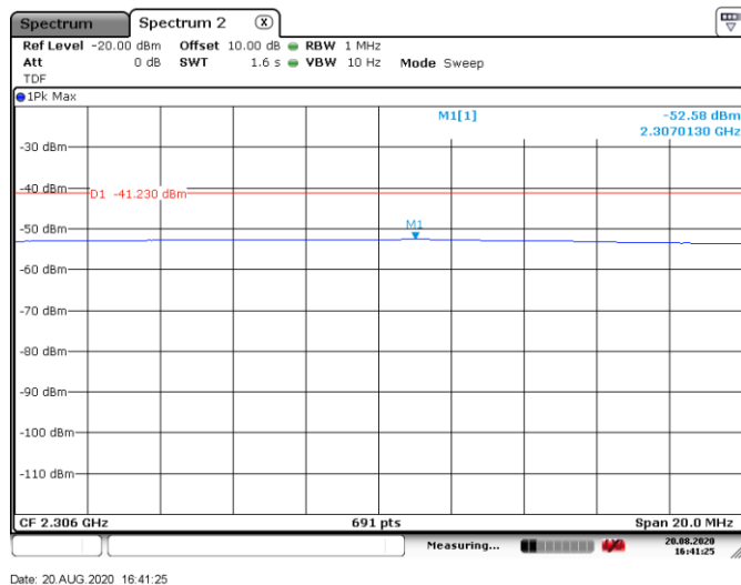
Figure 8.6-20: Conducted spurious emissions, tx on mid channel
