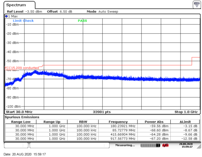
Figure 8.6-11: Conducted spurious emissions 30 MHz to 1 GHz within restricted bands, tx on mid channel
