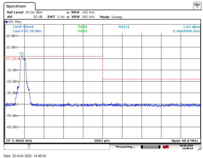
Figure 8.6-2: Band edge spurious emissions at 2483.5 MHz
