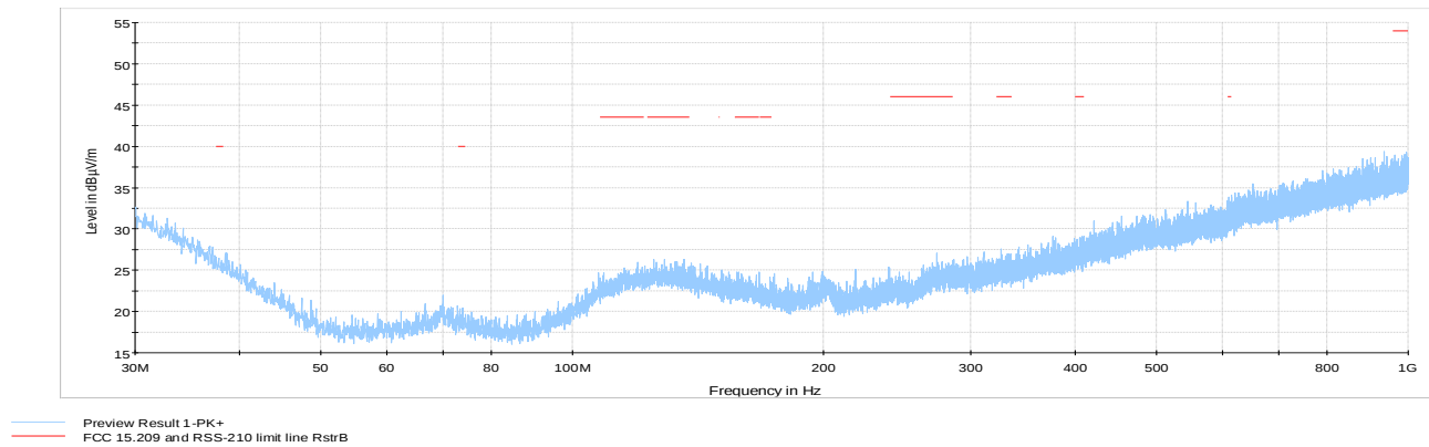
Figure 8.6-22: Cabinet radiated Spurious emissions within 30 to 1000 MHz, Tx @ low channel
