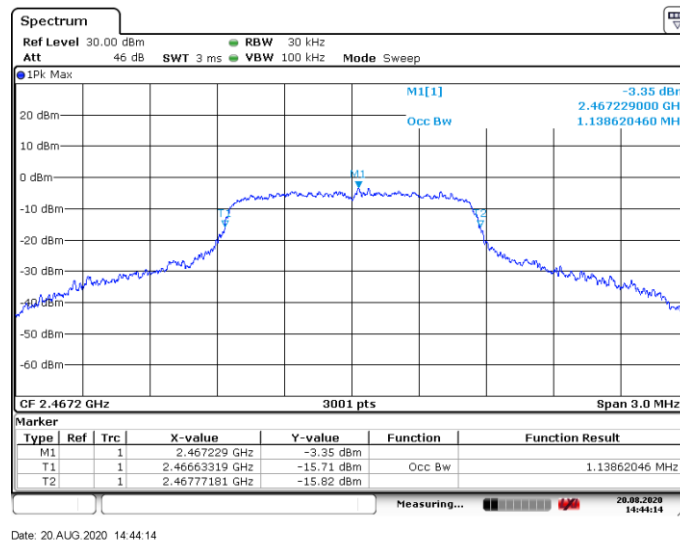
Figure 8.4-6: 99% occupied bandwidth on high channel
