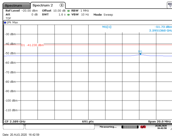
Figure 8.6-21: Conducted spurious emissions, tx on mid channel
