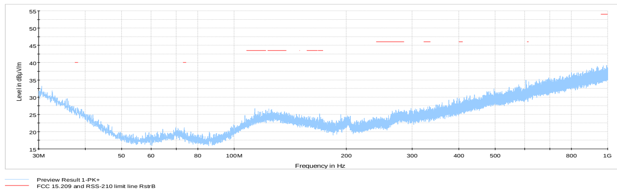
Figure 8.6-24: Cabinet radiated Spurious emissions within 30 to 1000 MHz, Tx @ high channel
