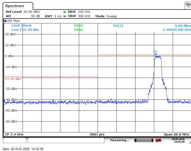
Figure 8.6-1: Band edge spurious emissions at 2400 MHz
