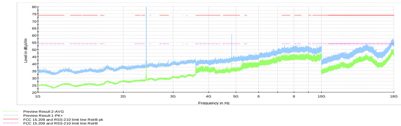
Figure 8.6-25: Cabinet radiated Spurious emissions 1to18 GHz, Tx @ low channel
