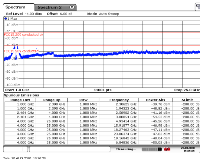
Figure 8.6-15: Conducted spurious emissions above 1 GHz within restricted bands, tx on high channel
