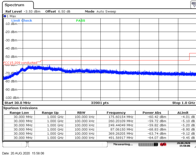
Figure 8.6-10: Conducted spurious emissions 30 MHz to 1 GHz within restricted bands, tx on low channel
