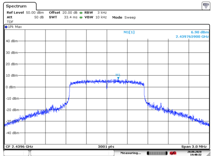
Figure 8.7-2: PSD on mid channel
