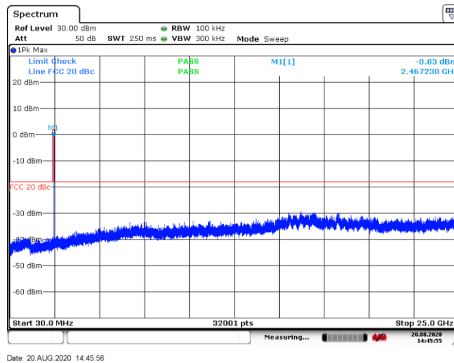
Figure 8.6-5: Conducted spurious emissions, tx on high channel
