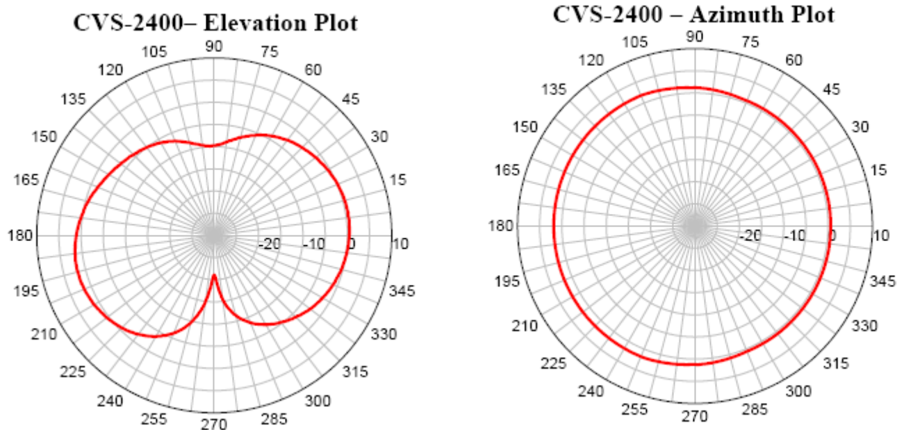
Figure 5: Mobile Mark CVS-2400 Radiation Patterns.
