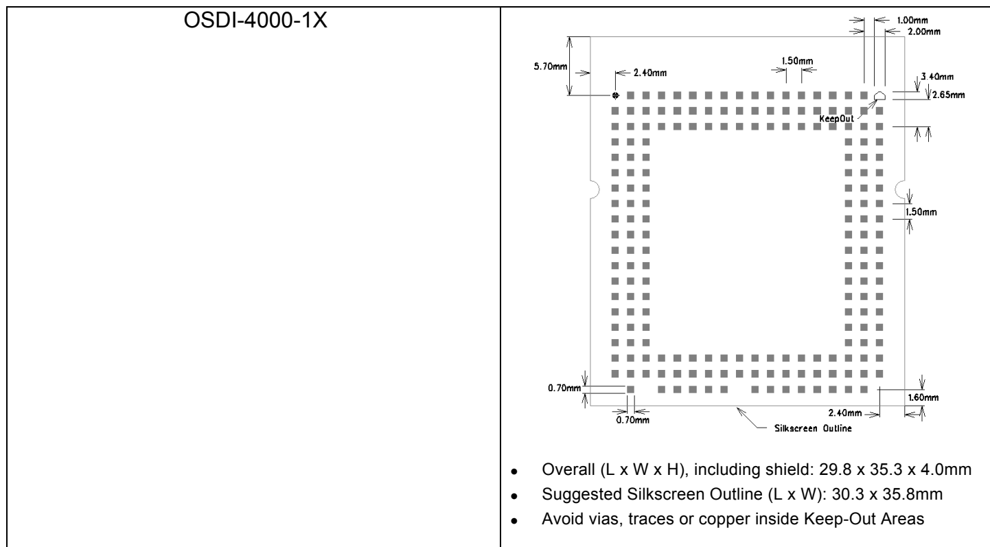
Figure 6 Footprint OSDI-4000-1X
