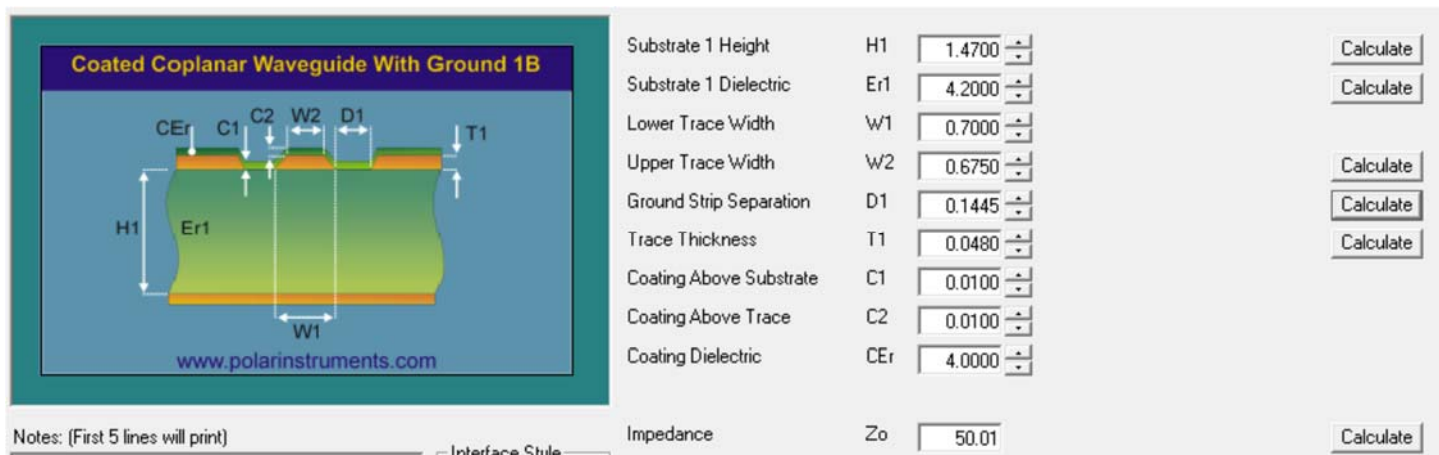
Figure 11: 50 ohms calculation (mm) Trace width: 0.7mm Copper clearance: 0.1445mm
