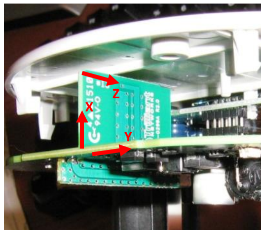
Figure 2: M Antenna orientation inside scanned product.
