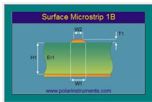
Figure 19: Micro-strip trace parameters
