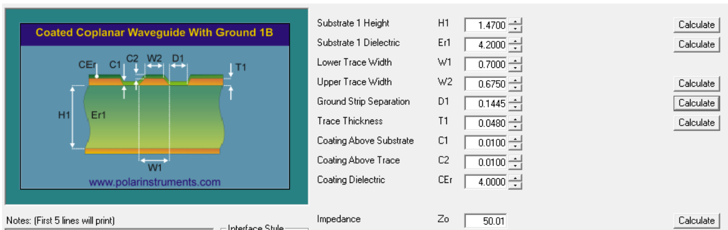
Figure 21: 50 ohms calculation (mm) Trace width: 0.7mm Copper clearance: 0.1445mm
