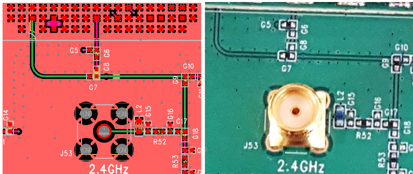
Figure 16 FCC and IC approved trace design layout and picture for external antennas of section 4.3
