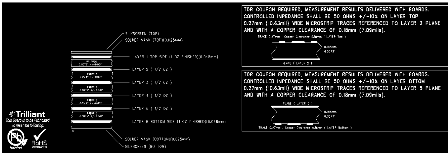
Figure 18 Coupon requirements to validate trace impedance
