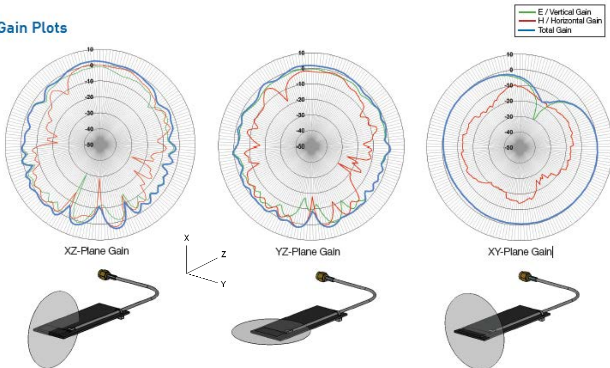
Figure 5: uSplat Antenna Radiation Patterns.
