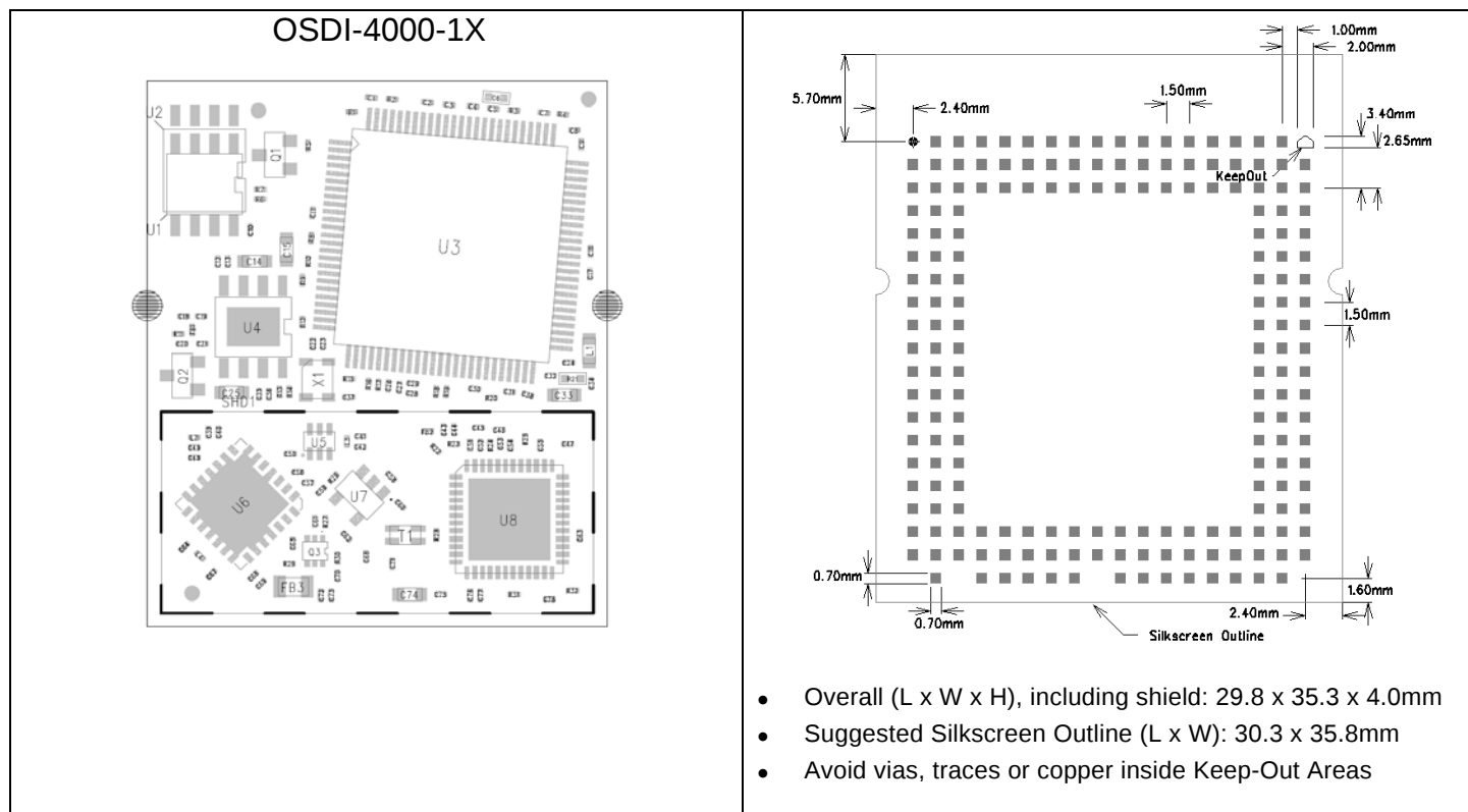
Figure 13 Footprint OSDI-4000-1X
