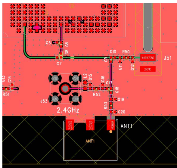
Figure 14 FCC and IC approved trace design layout and picture for the M antenna of section 4.2.1
