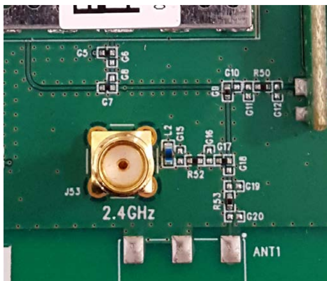
Figure 14 FCC and IC approved trace design layout and picture for the M antenna of section 4.2.1
