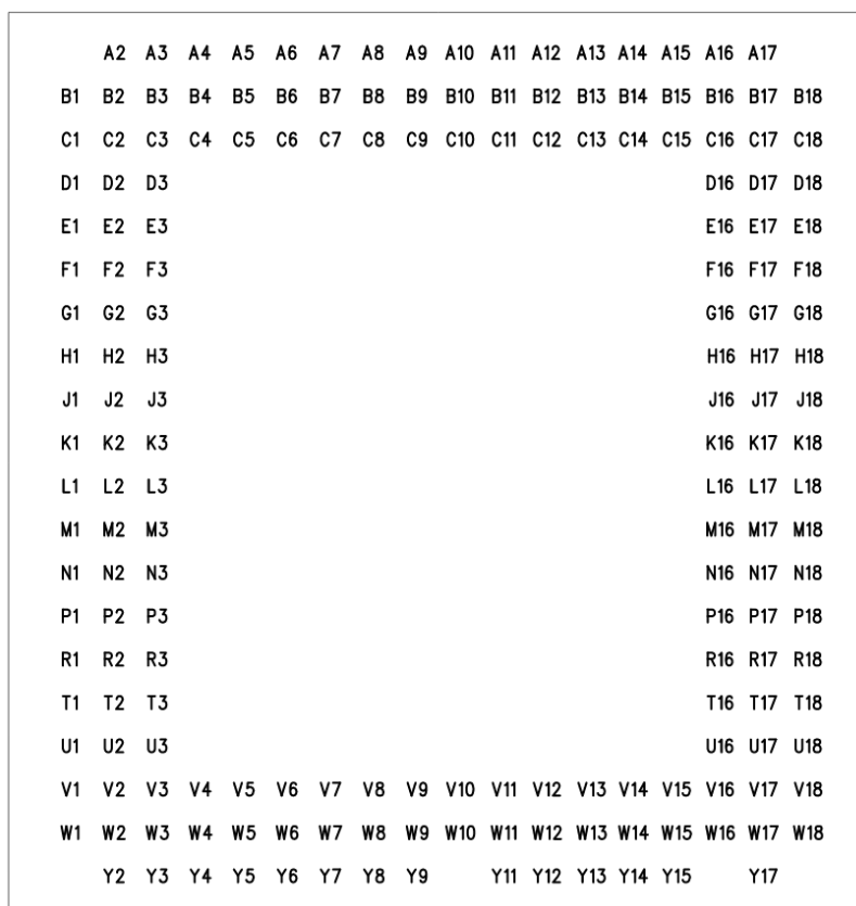
Figure 22: Pin Numbering Diagram Bottom view
