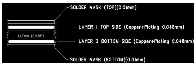
Figure 20: Example stack-up
