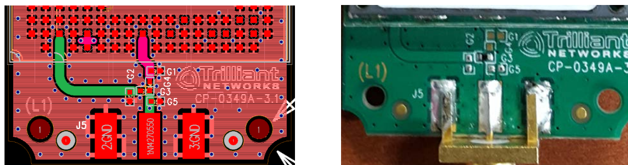
Figure 17 FCC and IC approved trace design layout and picture for external antennas of section 4.3
