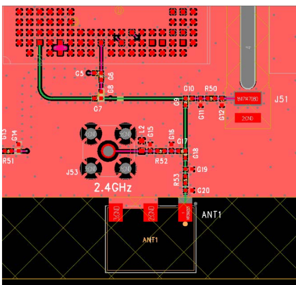
Figure 15 FCC and IC approved trace design layout and picture for the uSplash antenna of section 4.2.2
