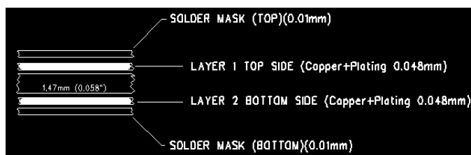
Figure 23: Example stack-up
