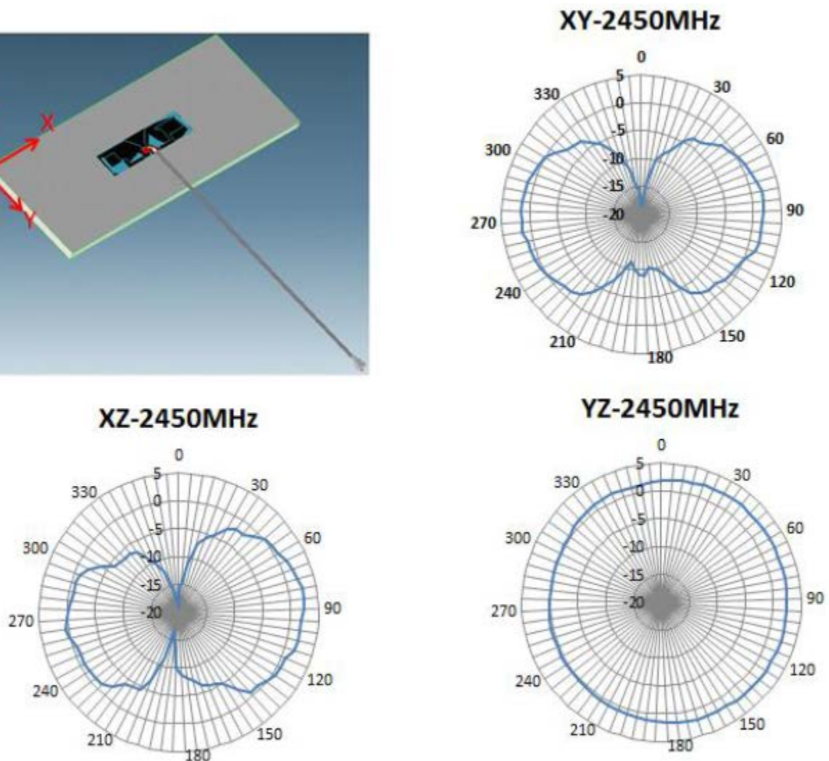
Figure 14 Molex 1461530100 Radiation Patterns.
