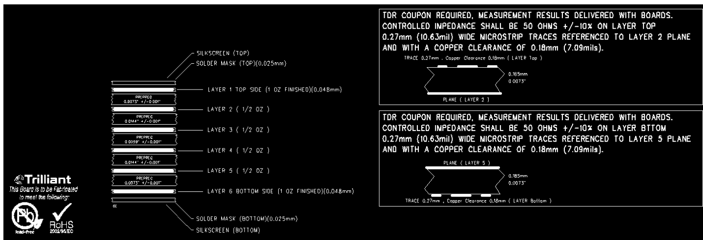
Figure 21 Coupon requirements to validate trace impedance
