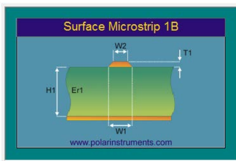
Figure 22: Micro-strip trace parameters
