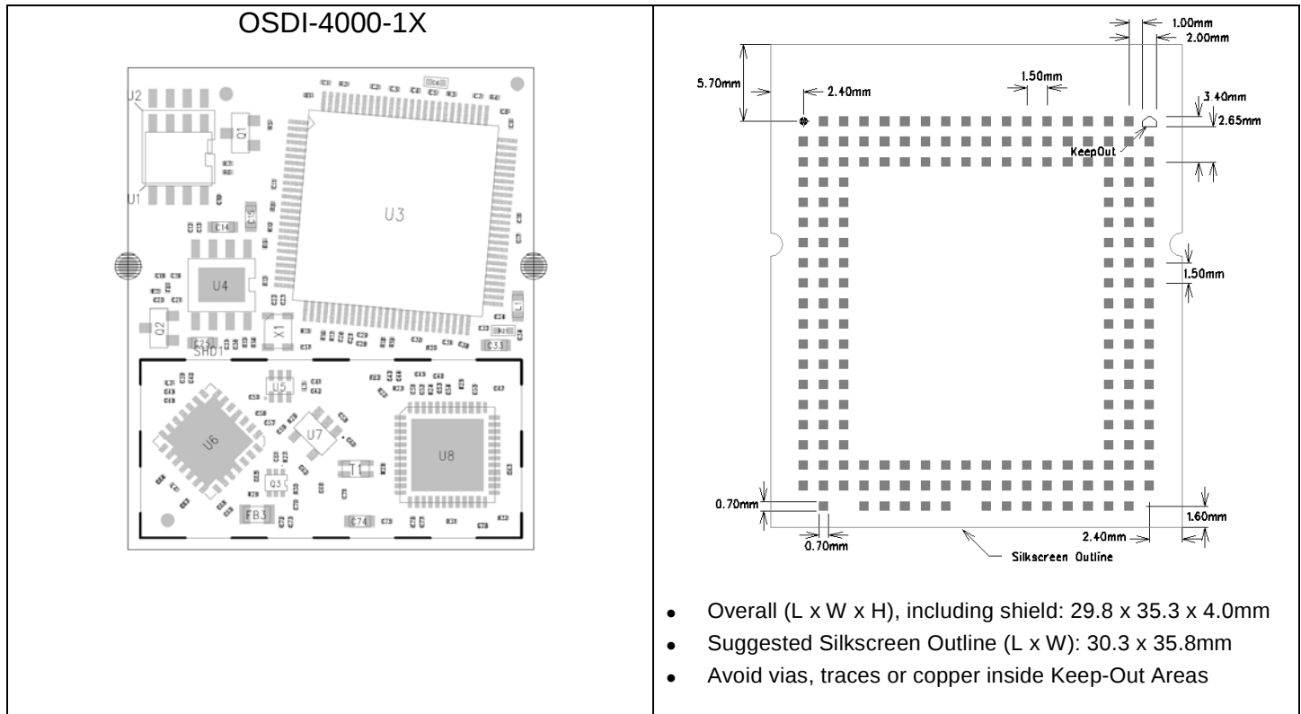
Figure 15 Footprint OSDI-4000-1X
