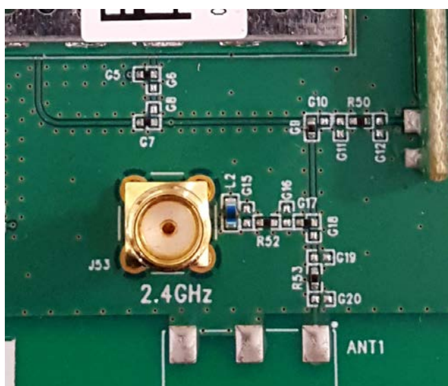
Figure 16 FCC and IC approved trace design layout and picture for the M antenna of section 4.2.1
