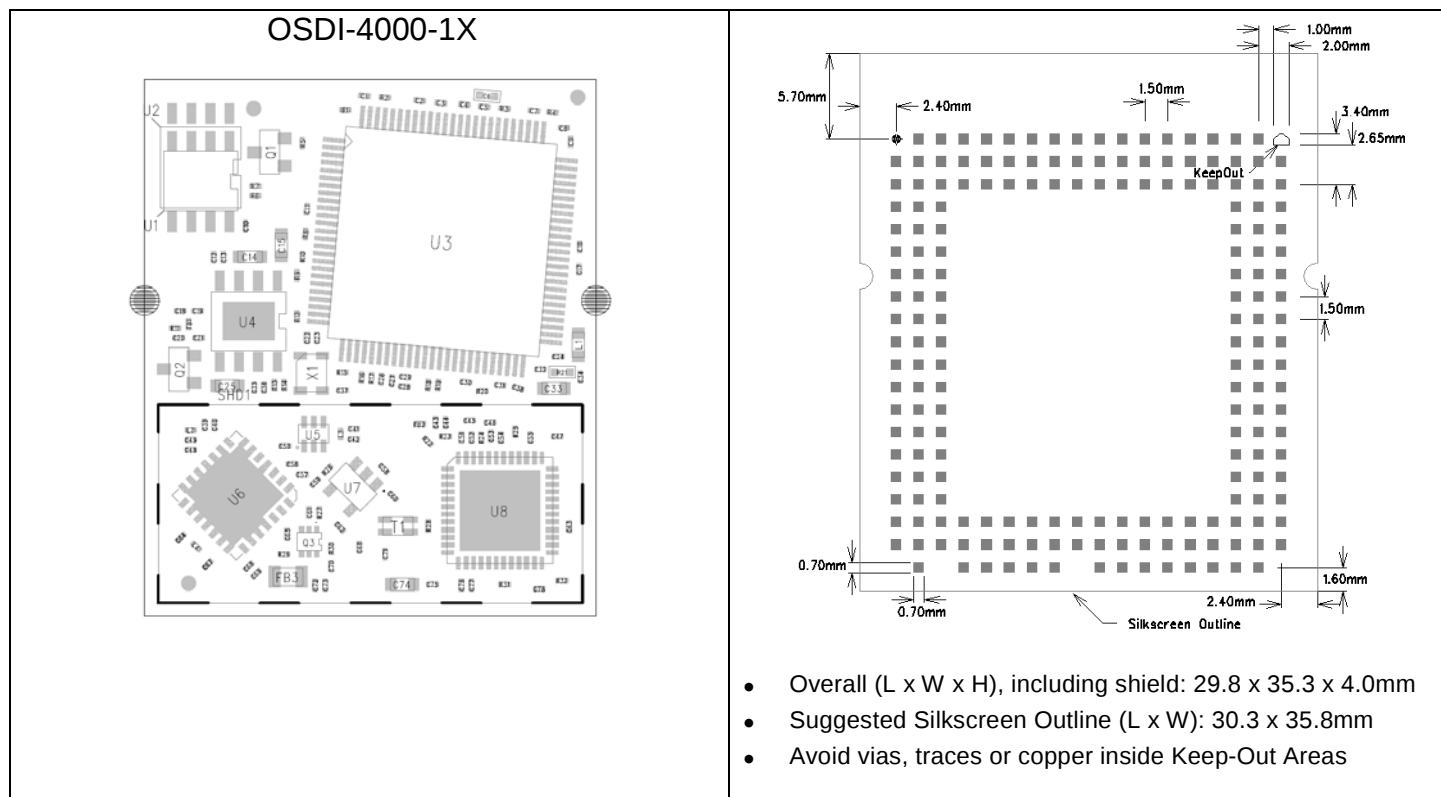
Figure 15 Footprint OSDI-4000-1X
