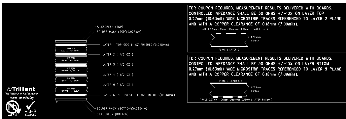
Figure 22 Coupon requirements to validate trace impedance
