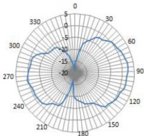
Figure 14 Molex 1461530100 Radiation Patterns.
