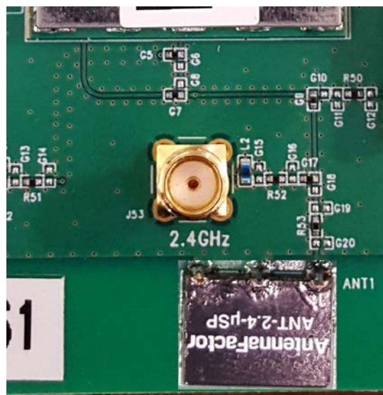
Figure 17 FCC and IC approved trace design layout and picture for the uSplash antenna of section 4.2.2
