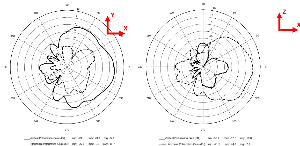
Figure 3 M Antenna Azimuth (left) and Elevation (right) Patterns.
