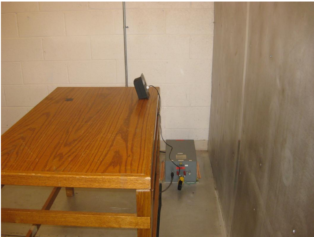
AC – Conducted #2
