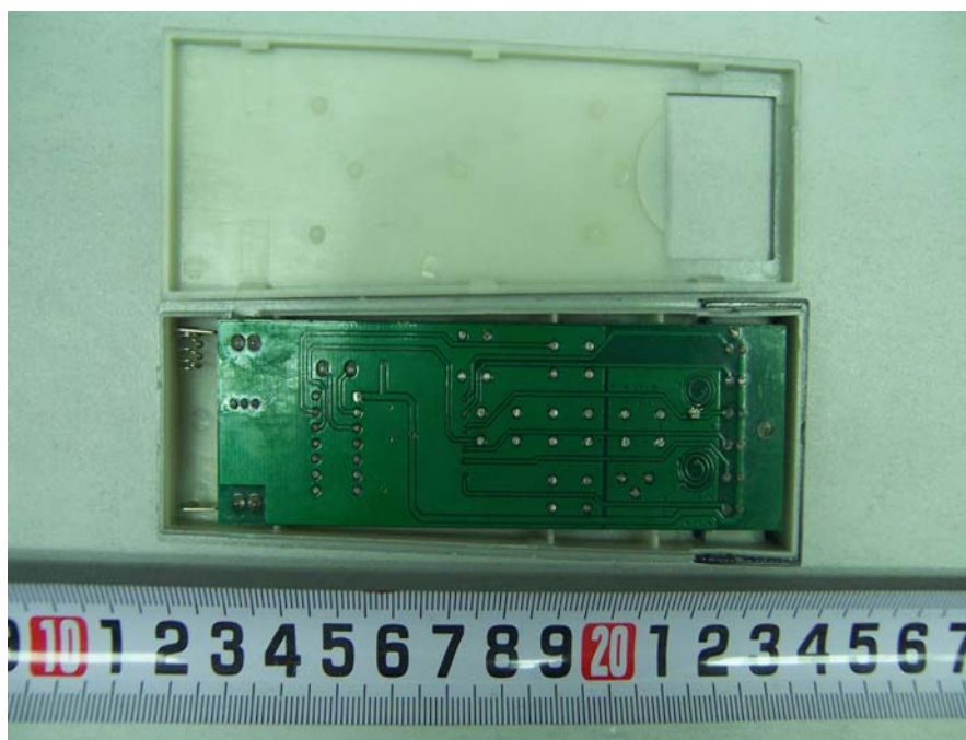
Uncovered View
