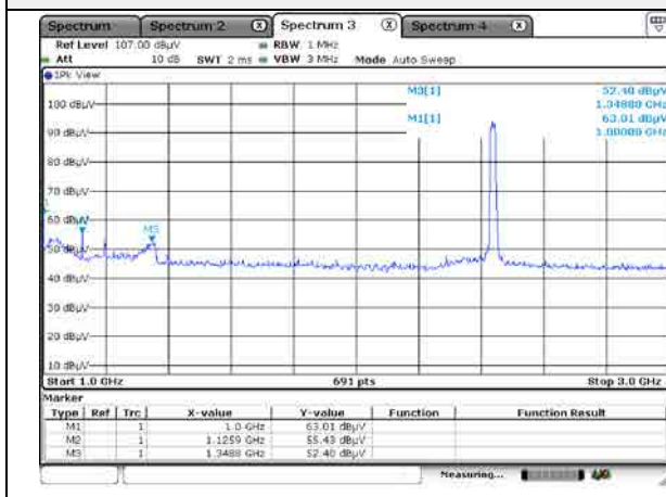
Horizontal // Peak for 1 GHz to 3 GHz
