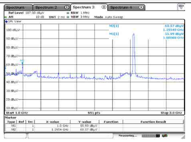
Vertical // Peak for 1 GHz to 3 GHz
