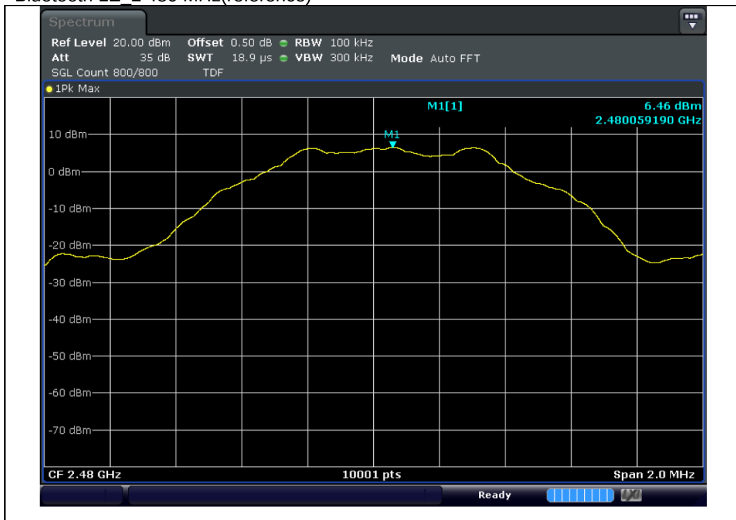
Bluetooth LE 2 480 MHz(reference)
