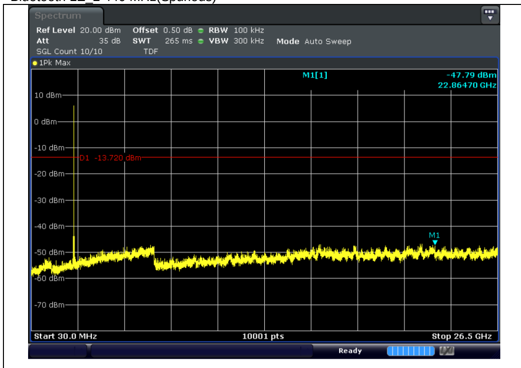
Bluetooth LE 2 440 MHz(Spurious)
