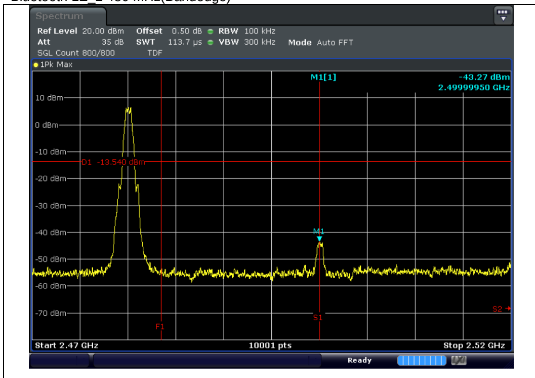
Bluetooth LE 2 480 MHz(Bandedge)
