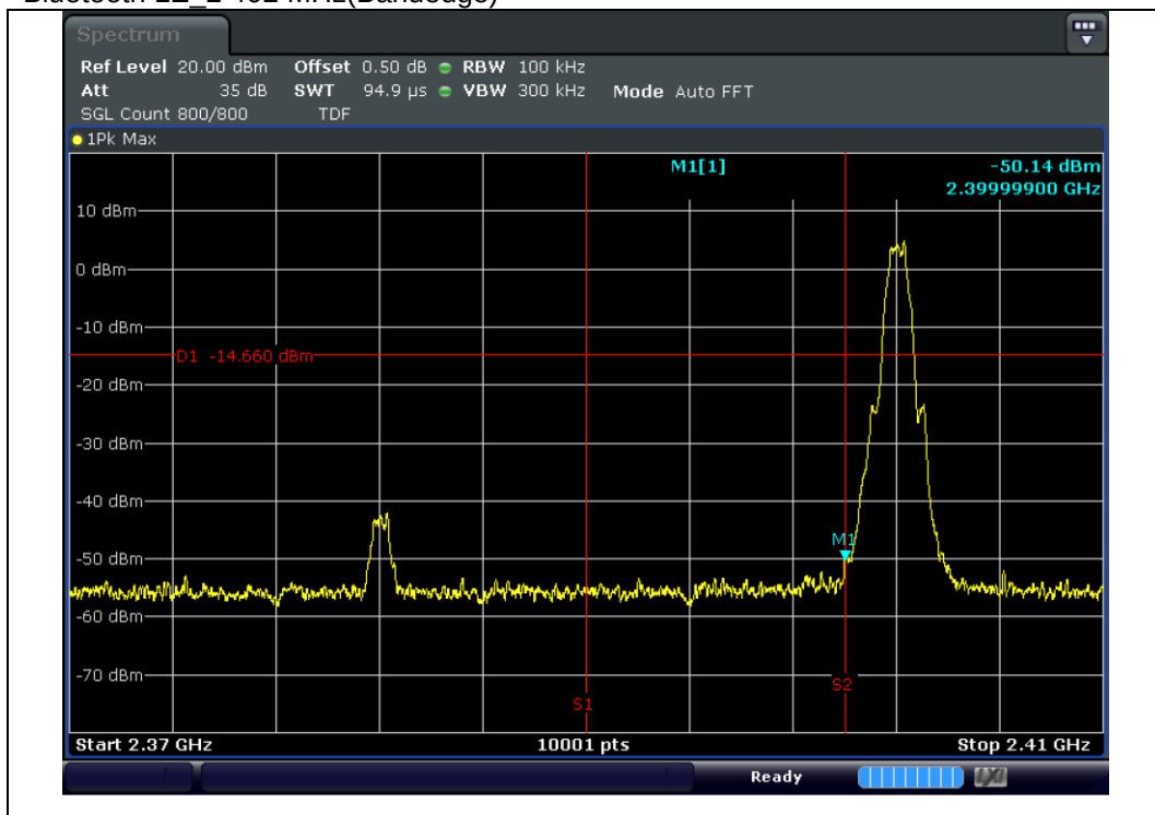
Bluetooth LE 2 402 MHz(Bandedge)
