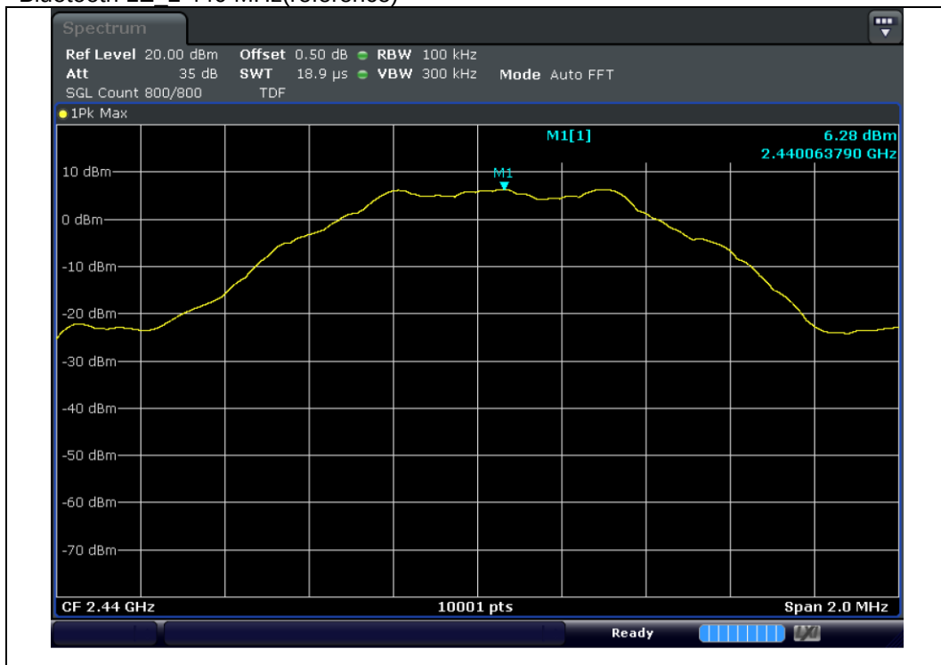
Bluetooth LE 2 440 MHz(reference)
