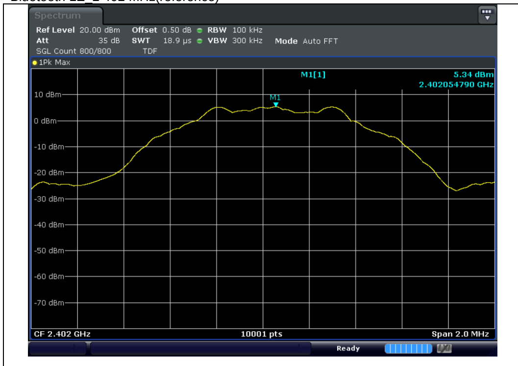
Bluetooth LE 2 402 MHz(reference)
