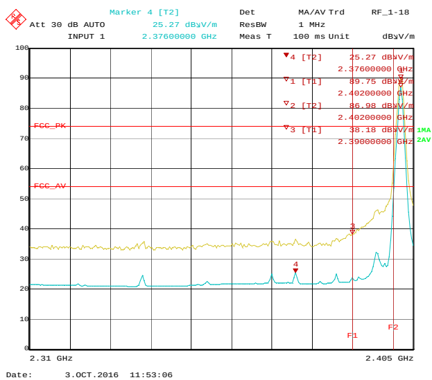
Figure 7. Plot of the Band Edge (Radiated) (DC 12 V)
