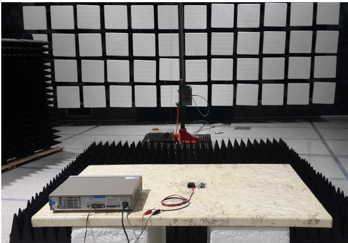
Radiated emission test above 18 GHz
