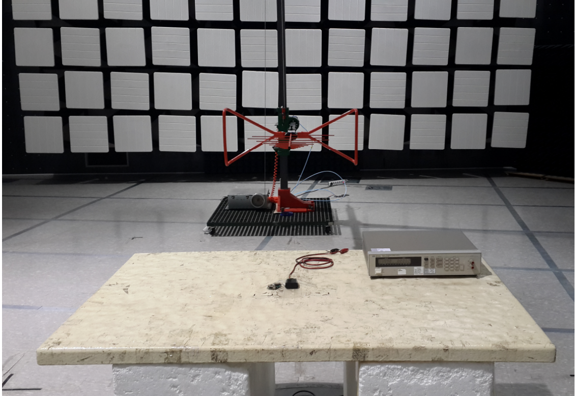
Radiated emissions - rear view
