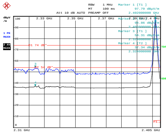
Figure 13. Plot of the Band Edge (Radiated)
