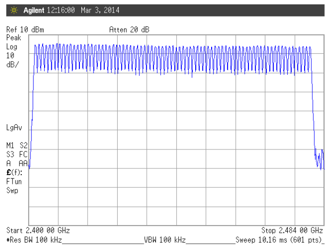
Figure 10. Plot of the Number of Hopping Channels
