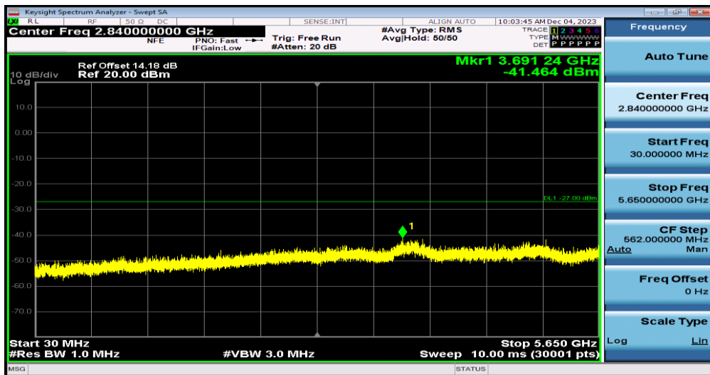
11N40MIMO-Ant1-5755-30~5650
