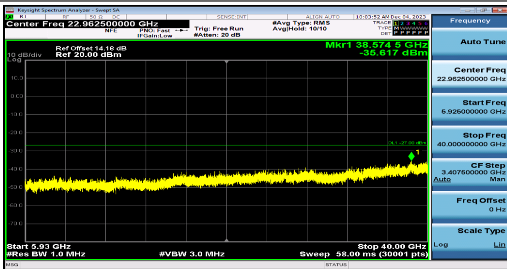
11N40MIMO-Ant1-5755-5925~40000
