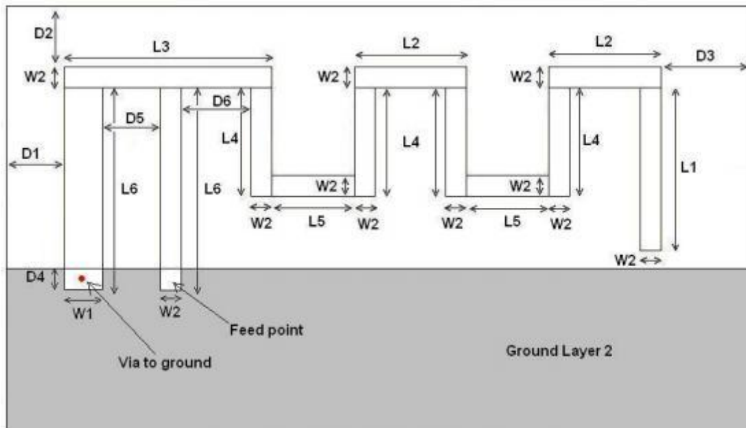
Figure 3: Antenna Dimensions
