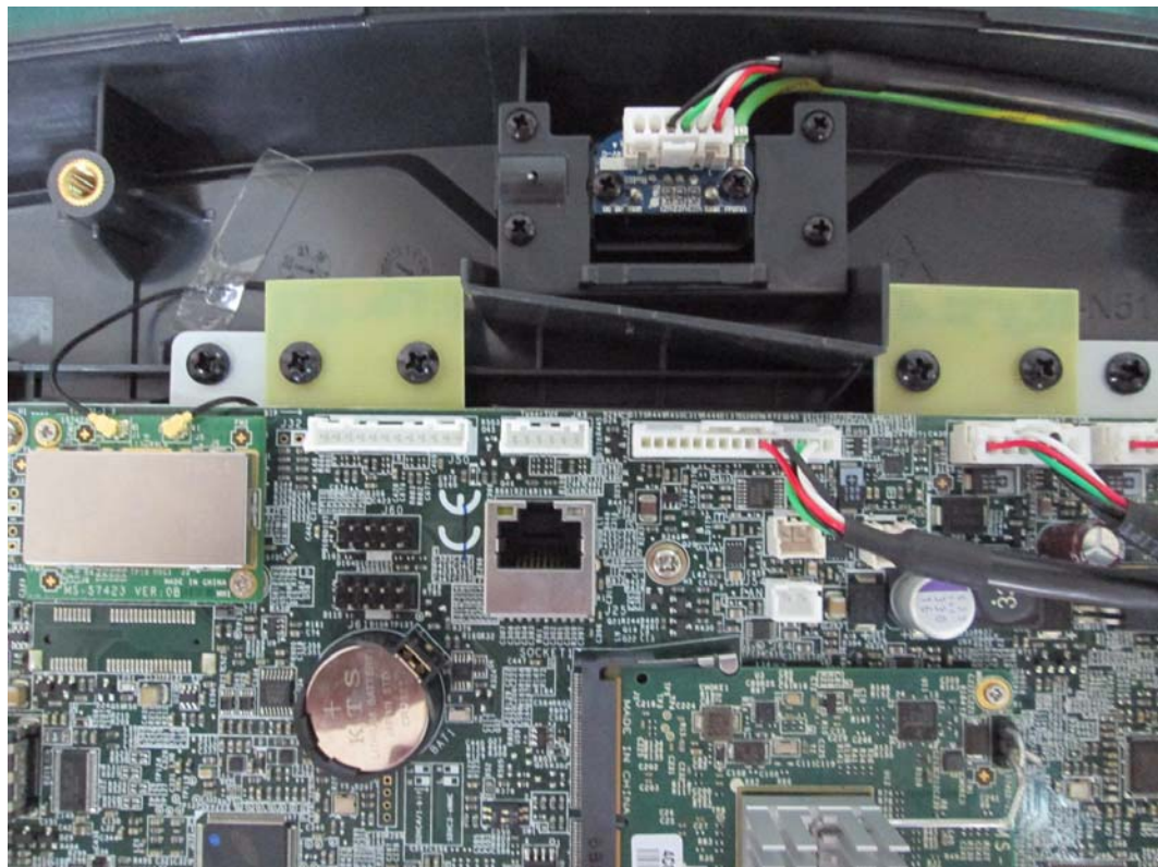
WiFi + BT module
