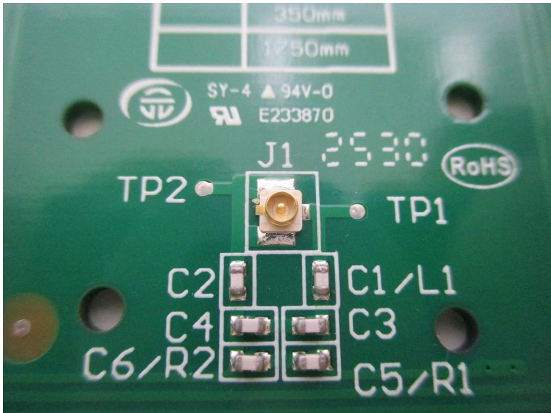
Antenna-IPEX
