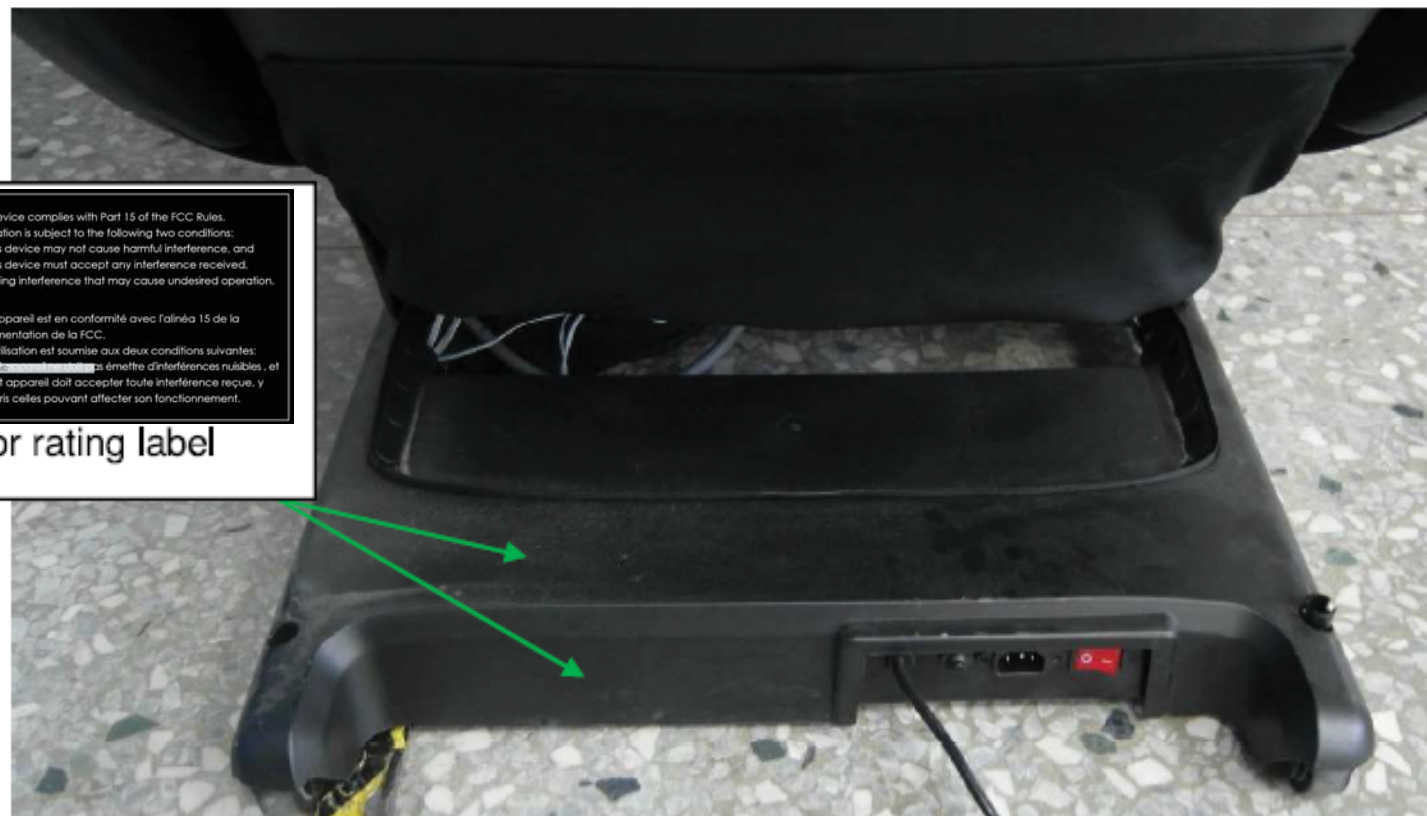
Location for circuit breaker, appliance inlet, and power switch
