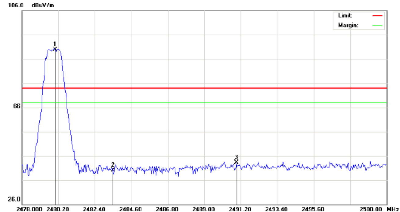
TEST PLOT OF BAND EDGE FOR HIGH CHANNEL (1Mbps)-Horizontal
