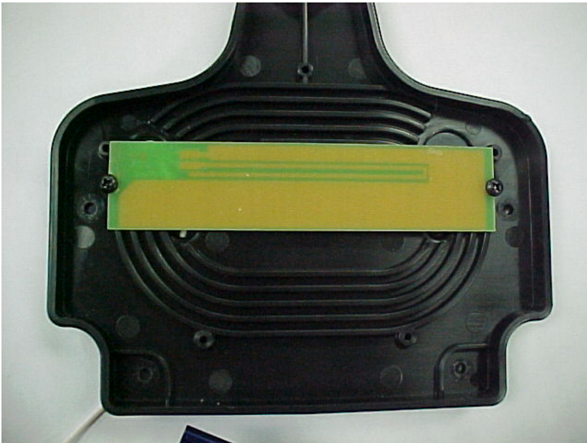
Photo Two – Internal Close Up of Antenna
