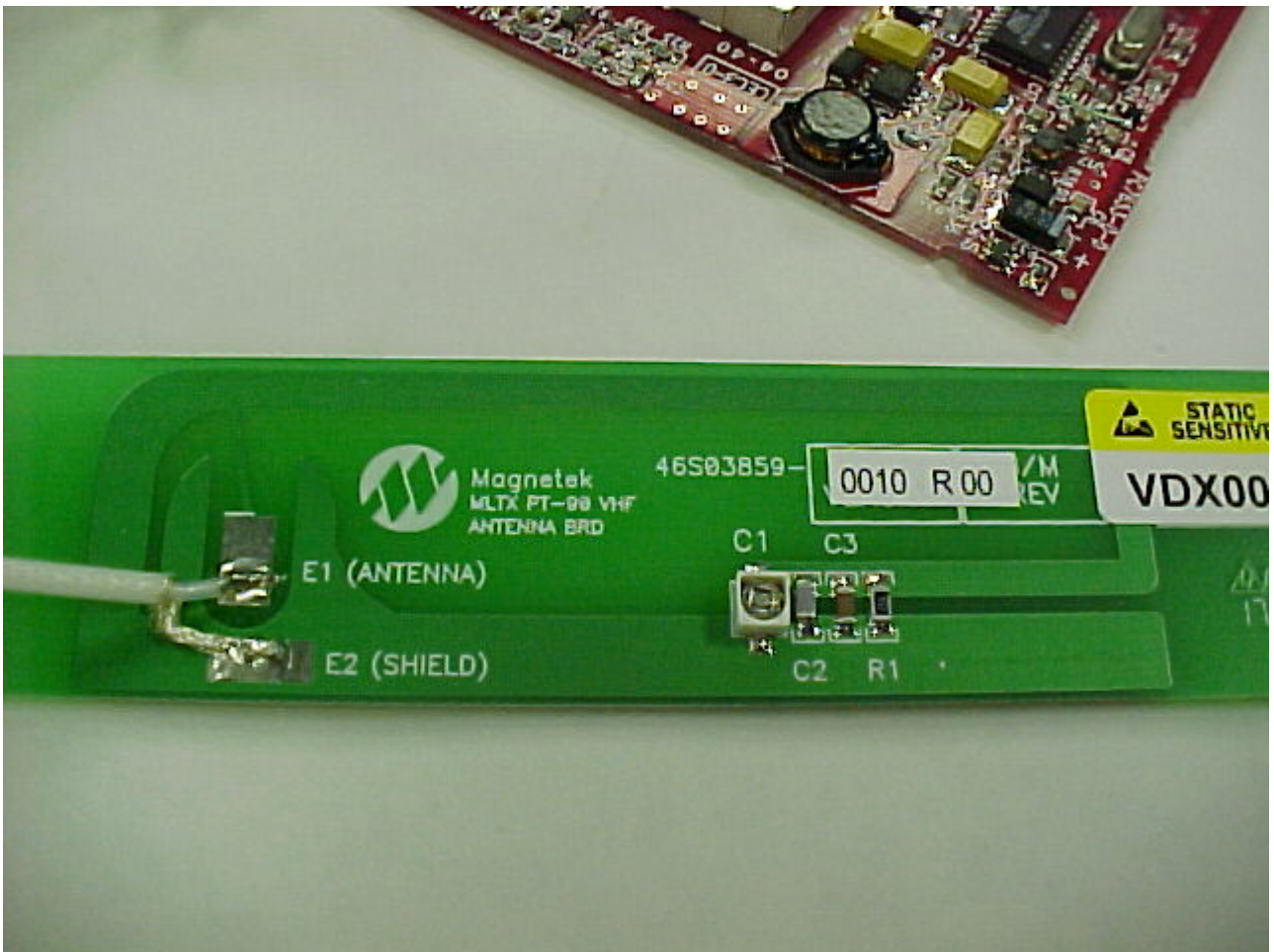
Photo Four – Internal Antenna Connection Close up
