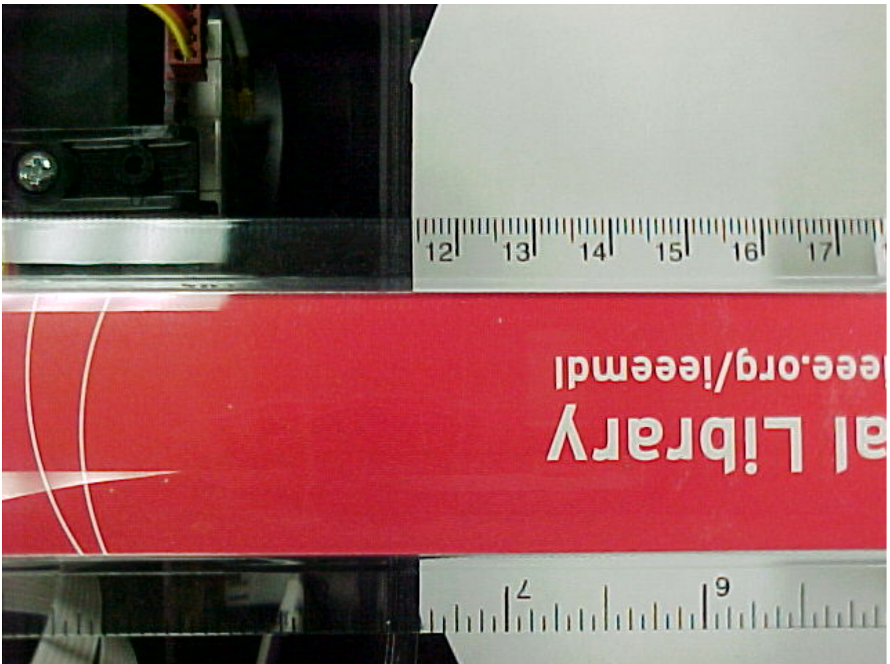
Photo Six – Internal Antenna Separation from Body
