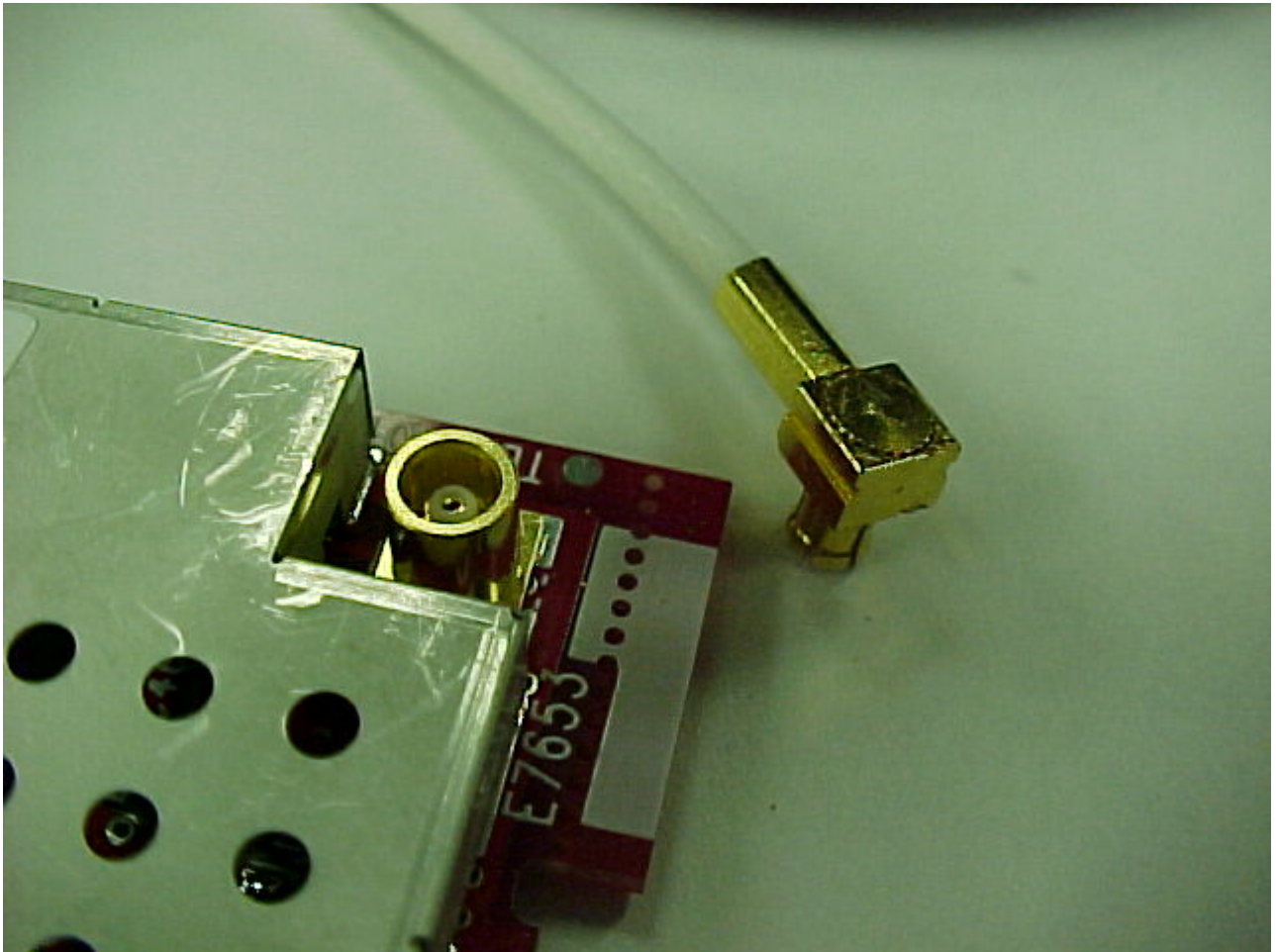
Photo Six – Internal Close Up of Antenna Lead Connector
