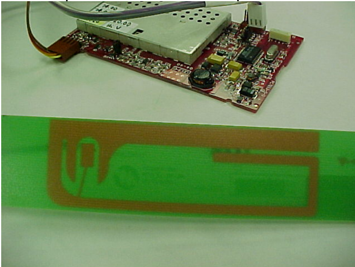
Photo Eight – Internal Component Side of PCB with Close-up of RF Section
