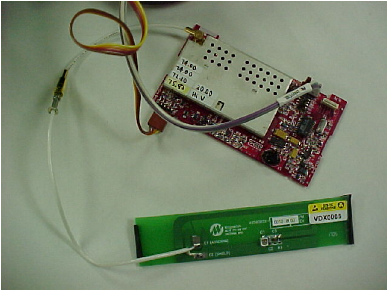
Photo Three – Internal RF Board Top with PCB Antenna Bottom
