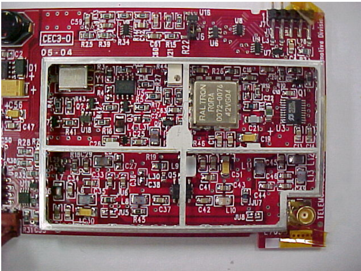
Photo Five – Internal Close Up of RF Board, Unshielded
