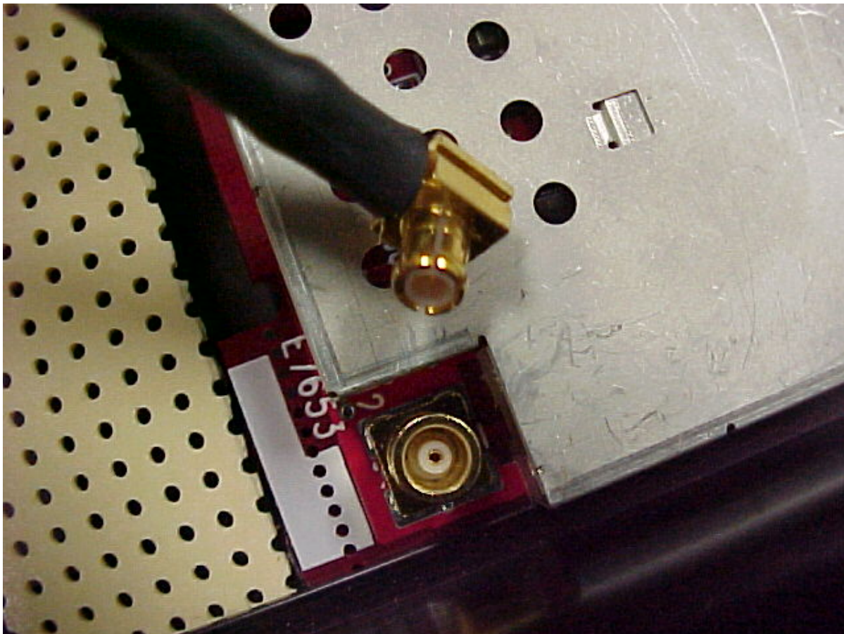
Photo Three – Internal Close Up of Antenna Connector
