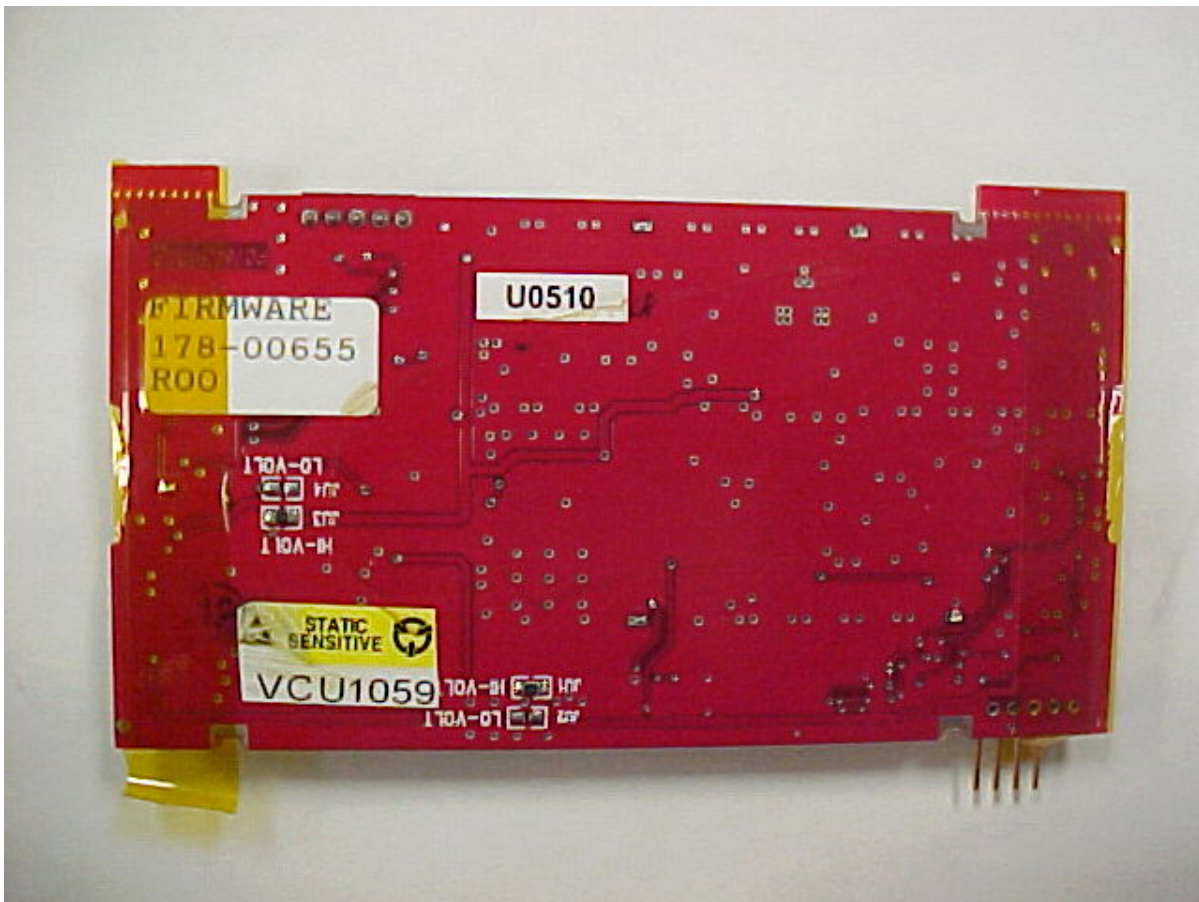
Photo Six – Internal Back of RF Board, No Components
