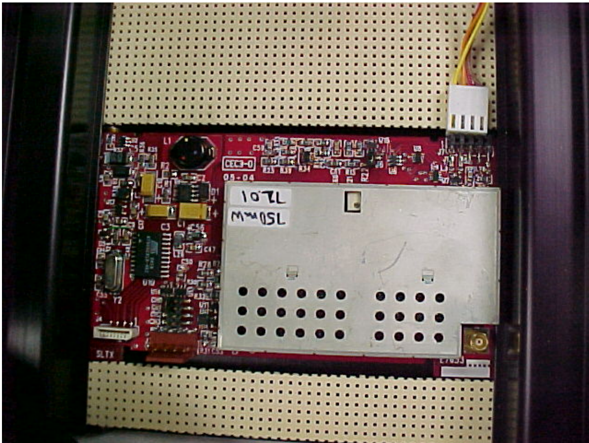
Photo Four – Internal Close Up of RF Board, Unshielded
