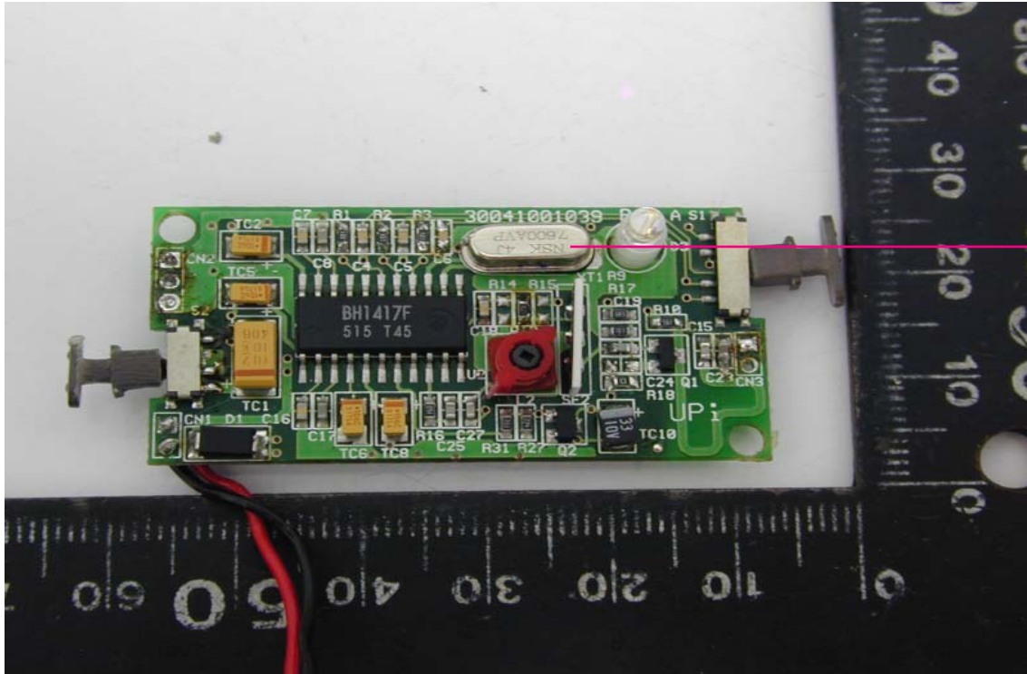
Component Side View of Main Board
