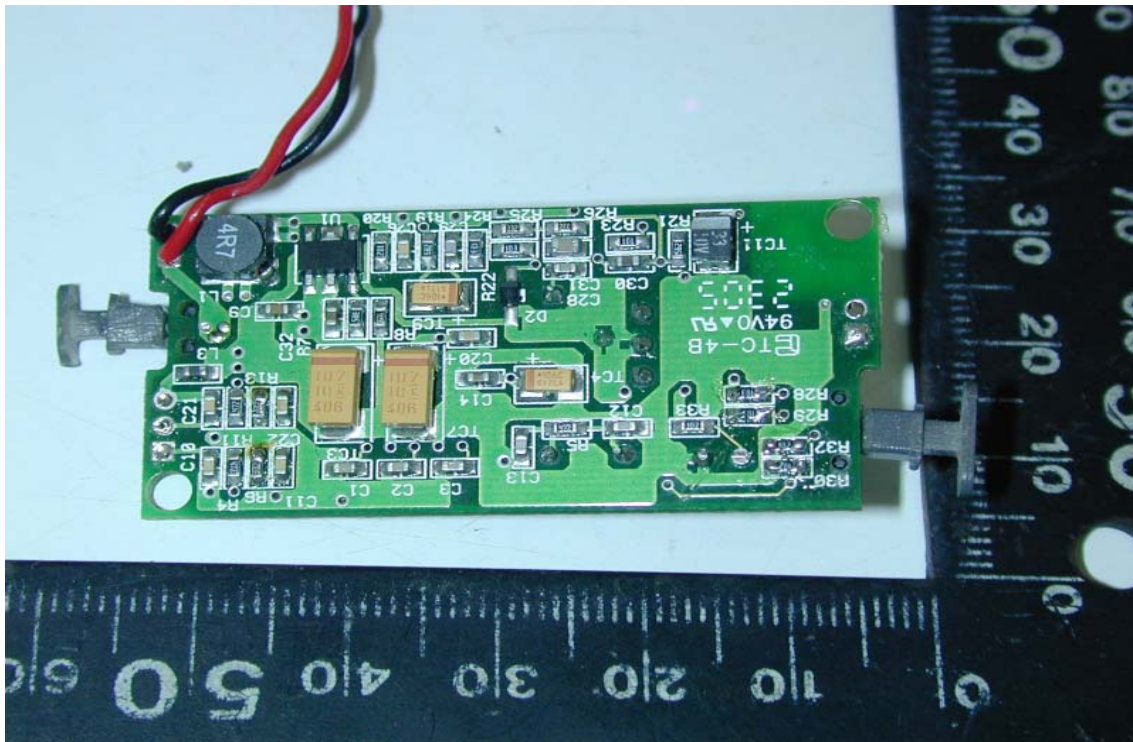
Solder Side View of Main Board
