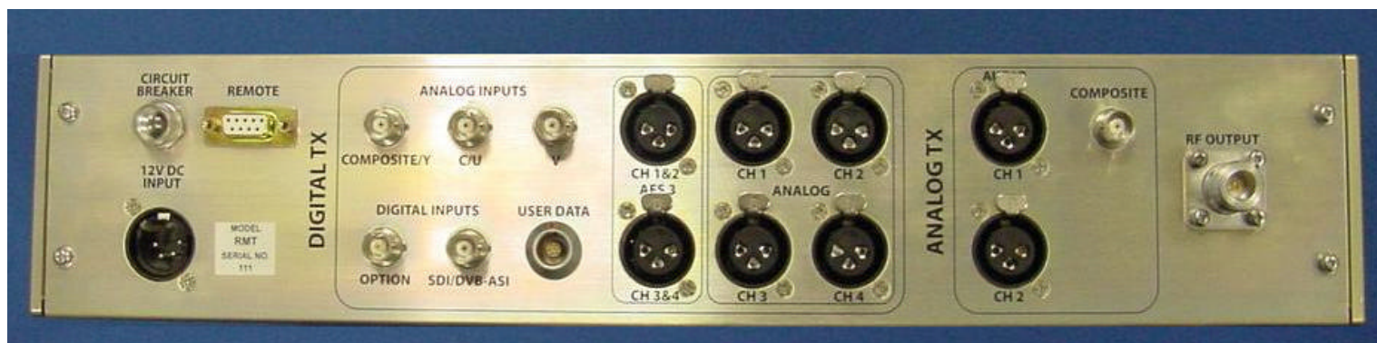
RMT Rear Panel layout showing all connections
