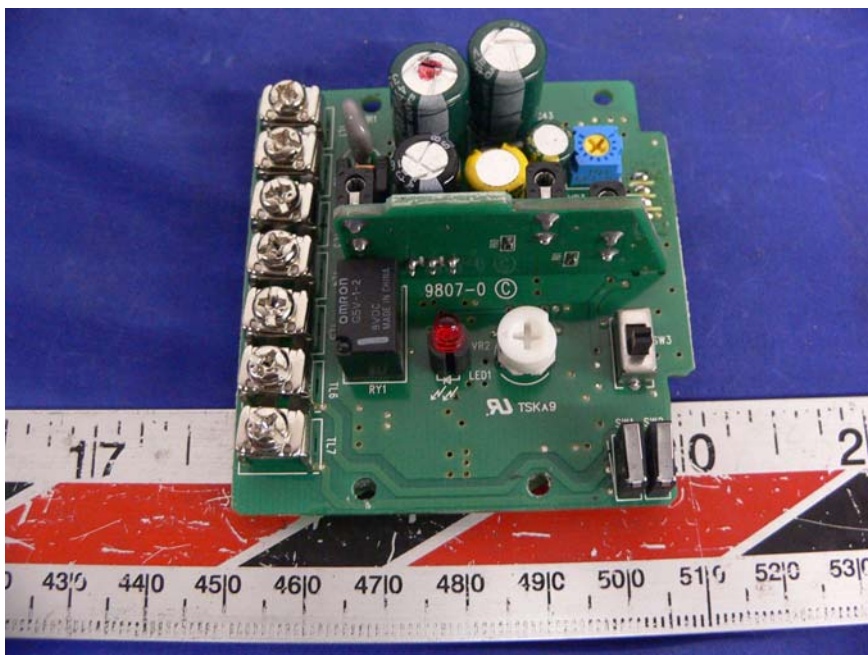
Receiver – Component View I
