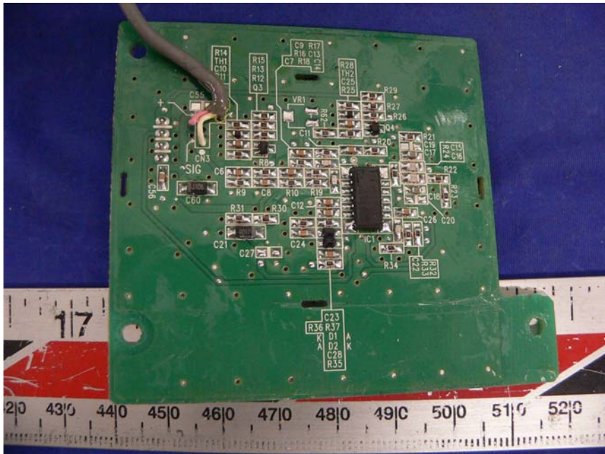
Receiver – Component View III
