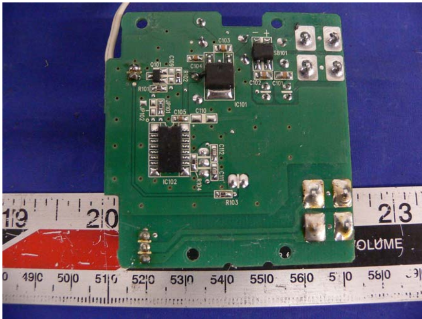
Transmitter – Component View II
