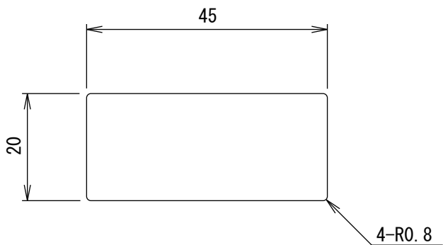
Trimming Die Drawing ( S = 1 / 1 )
