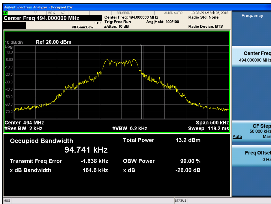
Occupied Bandwidth Plot (494.00 MHz)
