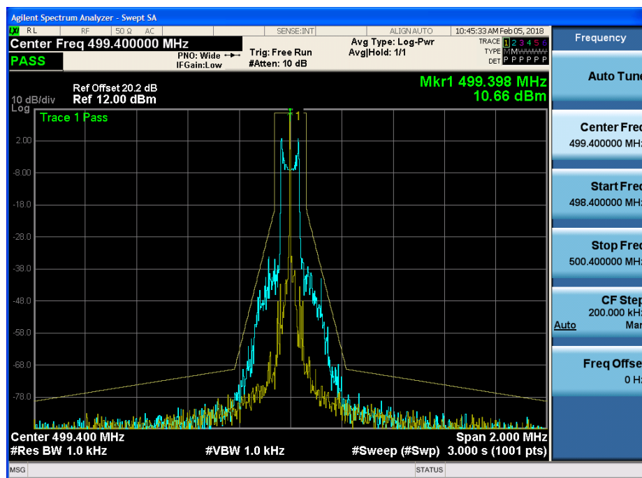
Emission mask Plot (499.40 MHz)
