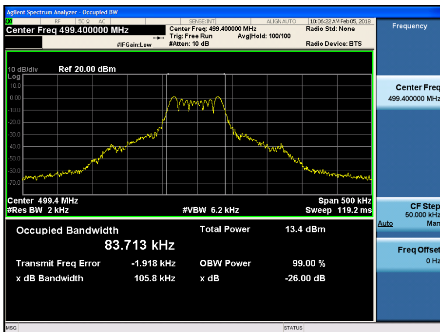
Occupied Bandwidth Plot (499.40 MHz)
