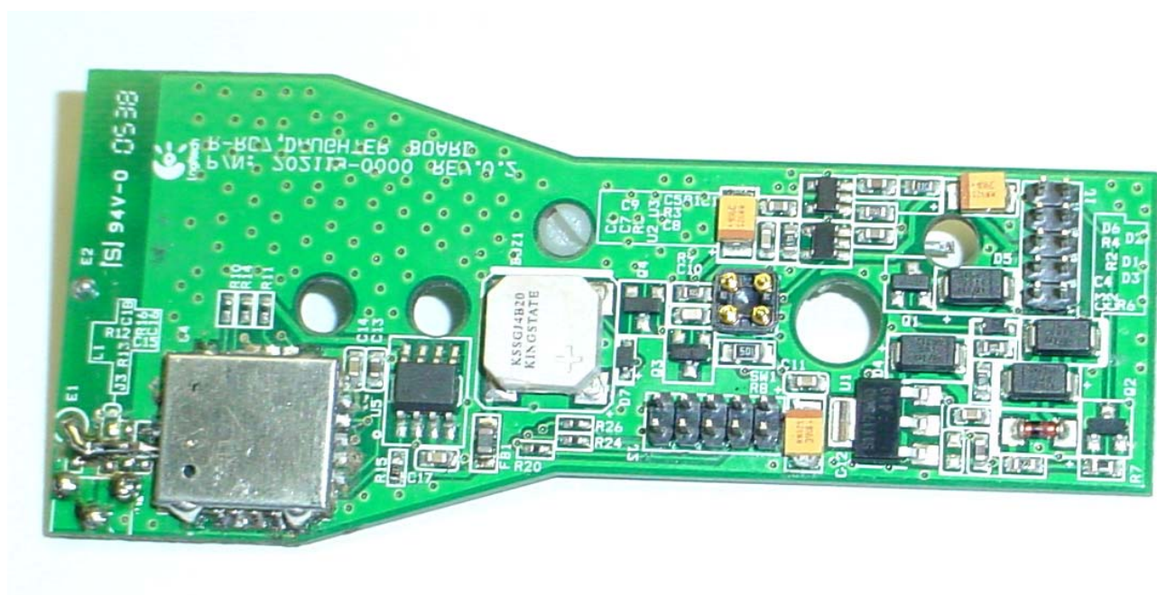
EUT with Cappuccino RF Daughter Antenna Board Top View
