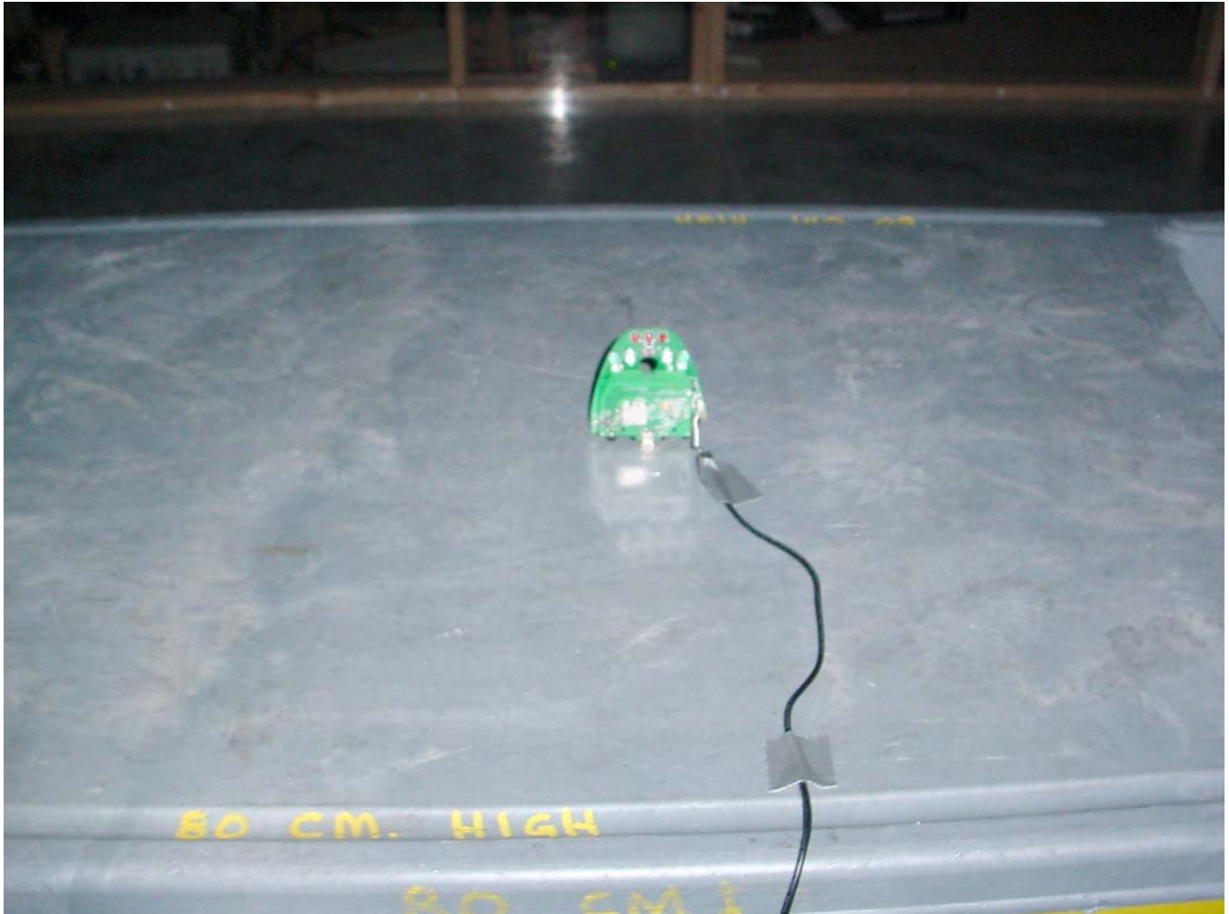
Radiated Emissions at 3 Meters EUT with Inverted F Antenna
