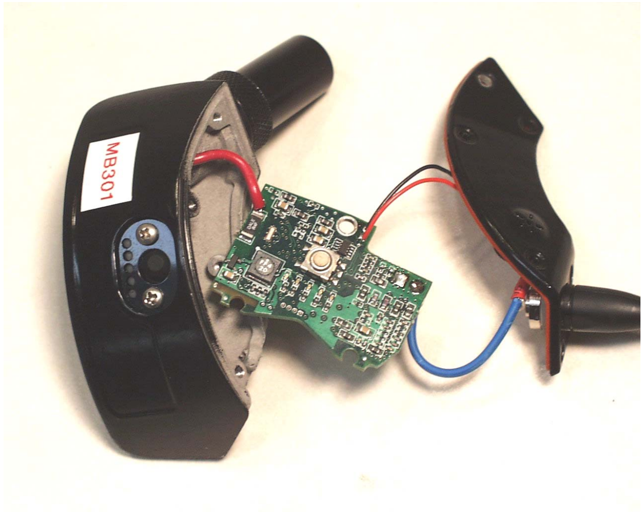
View of the Front Side of the PCB
