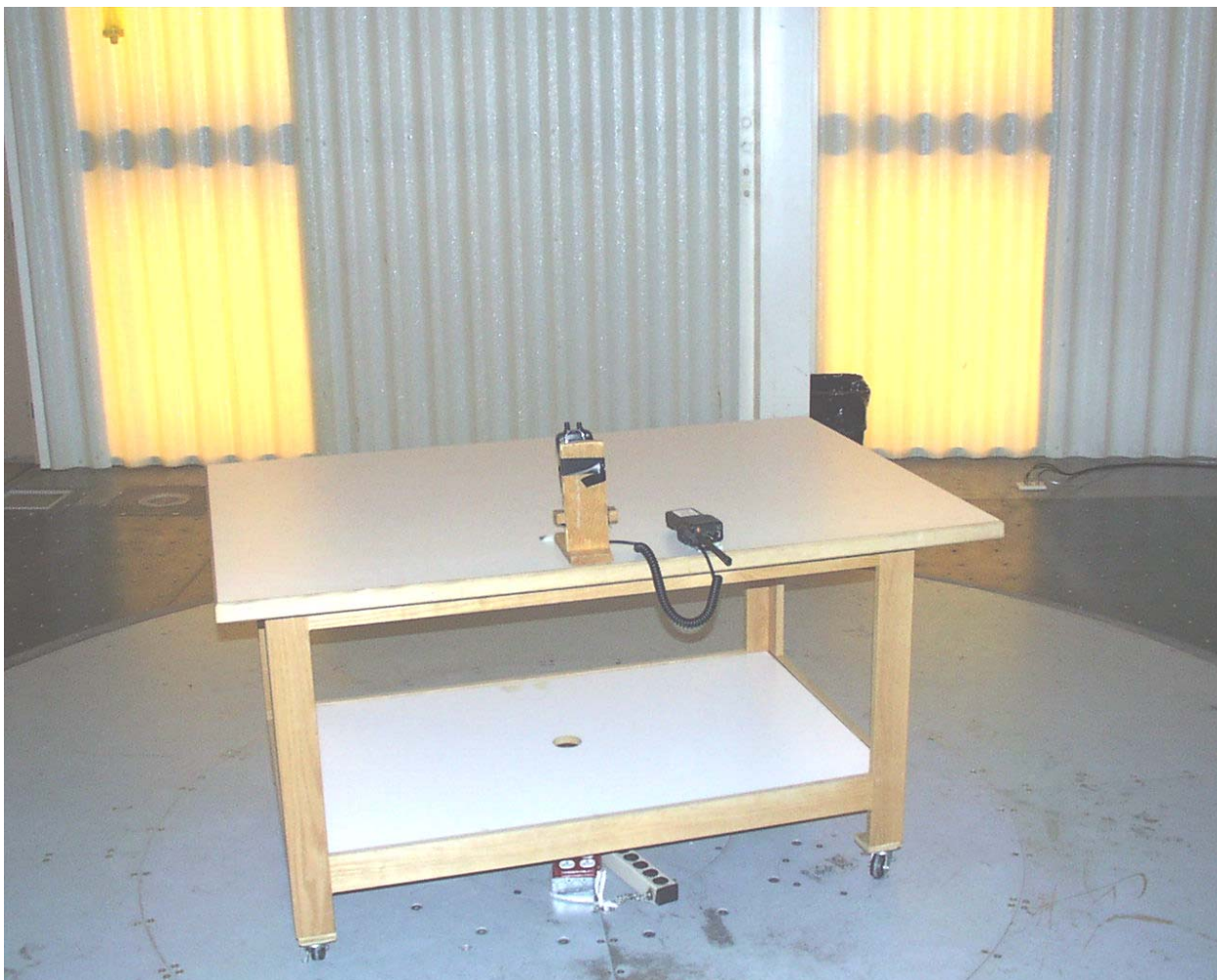
Back View of the Test Setup (Vertical Alignment)
