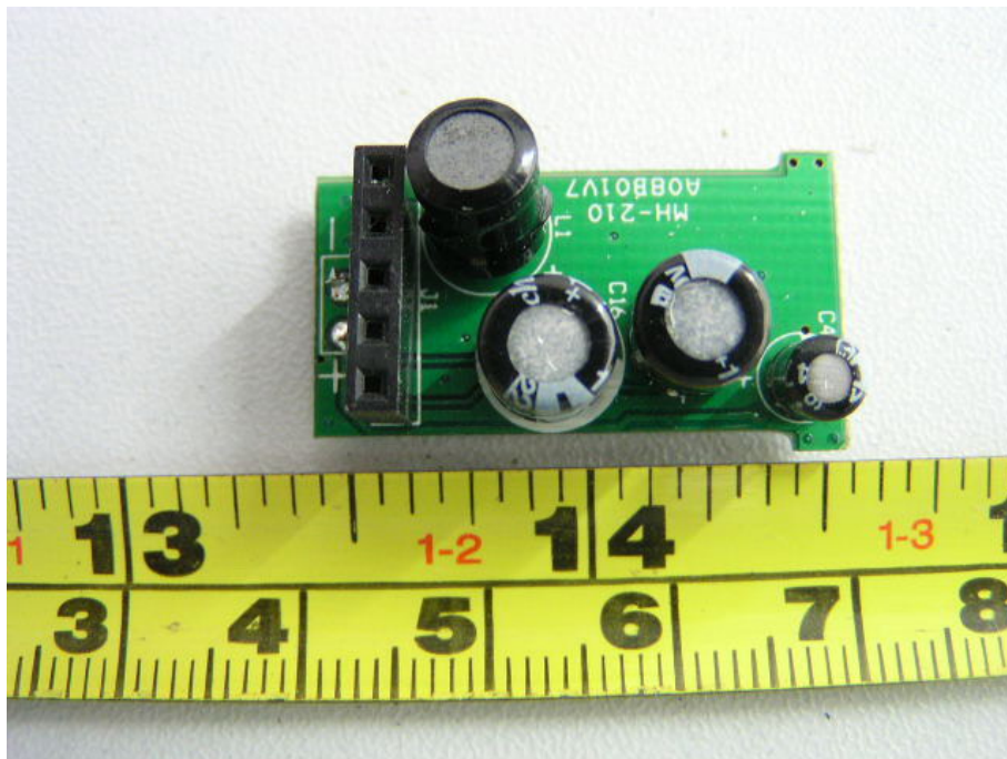
EUT – Top View of PCB (2)
