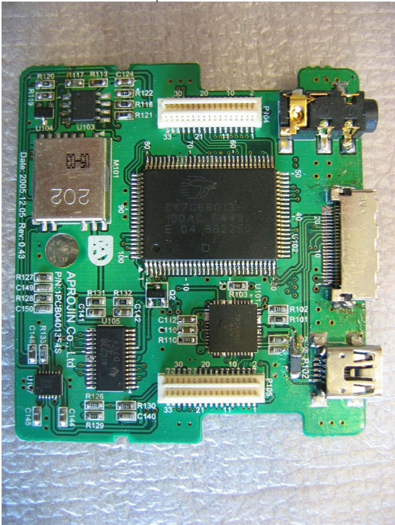
Top of interface board side
