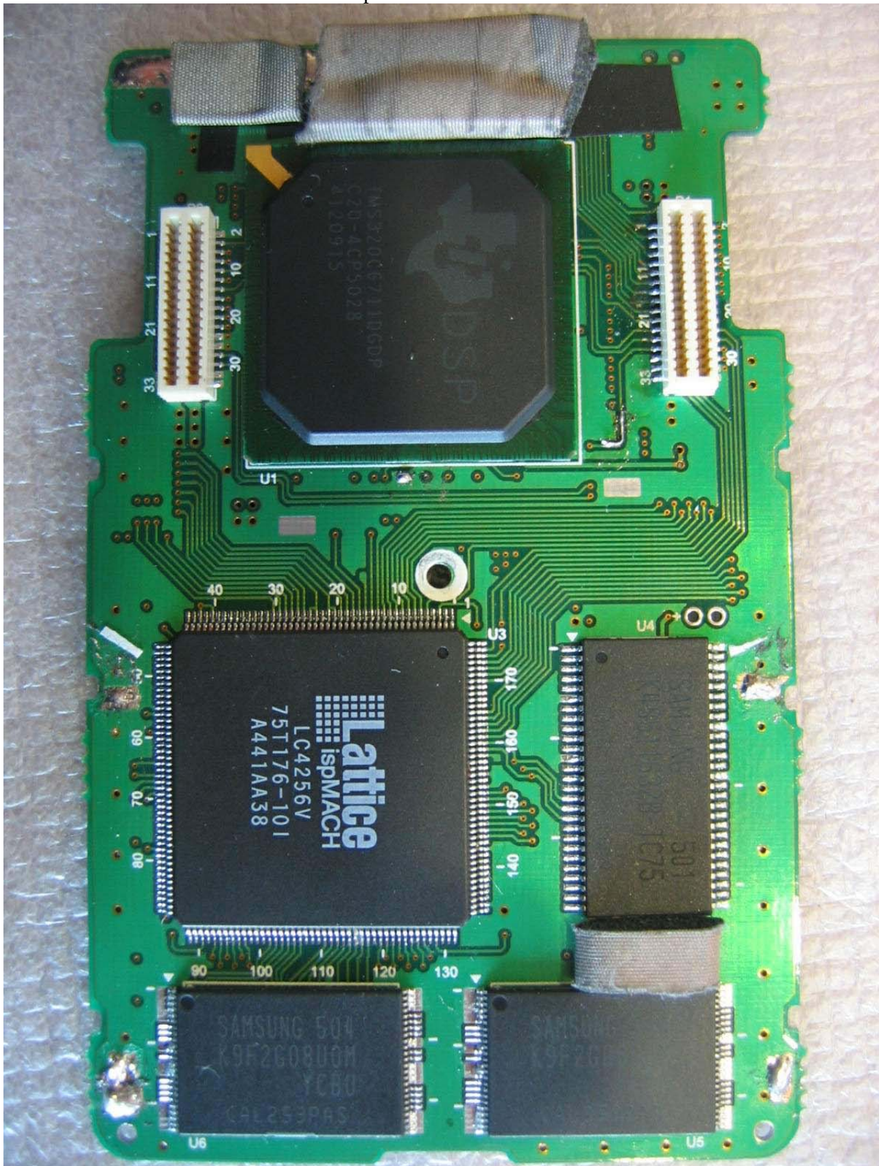
Top of main board side
