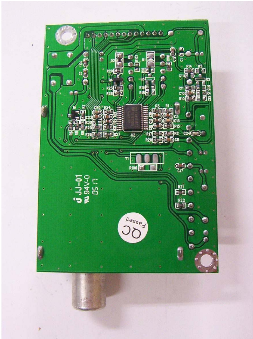
Board II Rear
